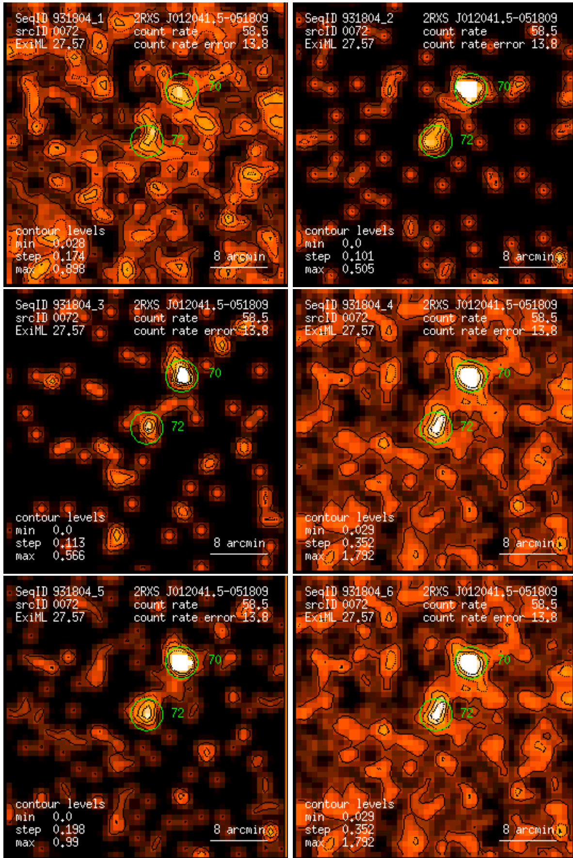
Figure 72: RASS 931804: detection 0072: band rate images, Gaussian filter: (1) PSPC channels 11 – 41, (2) 52 – 90, (3) 91 – 201, (4) 11 – 235, (5) 52 – 201, (6) 11 – 201. Broad band rates in counts/ks. Band rate contour levels in counts/ks/arcmin 2 .
