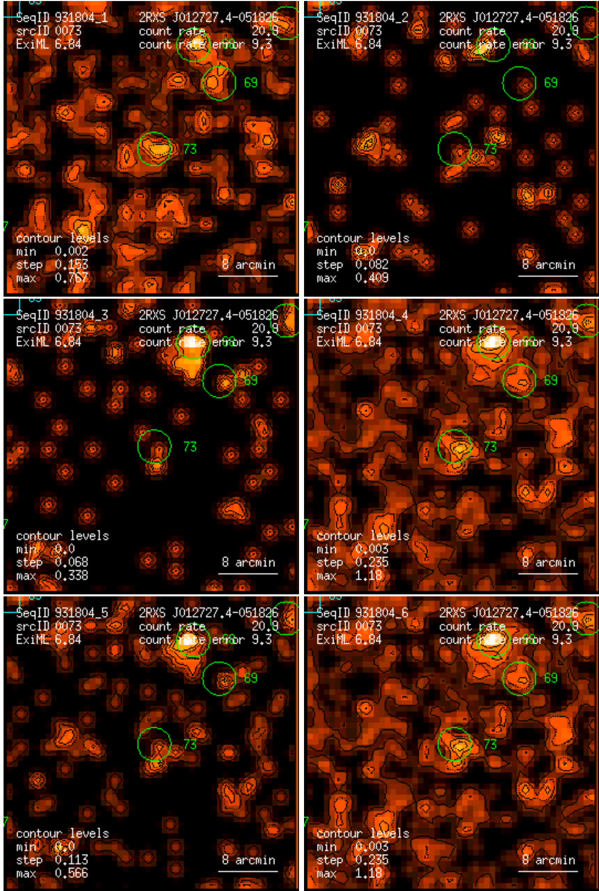
Figure 73: RASS 931804: detection 0073: band rate images, Gaussian filter: (1) PSPC channels 11 – 41, (2) 52 – 90, (3) 91 – 201, (4) 11 – 235, (5) 52 – 201, (6) 11 – 201. Broad band rates in counts/ks. Band rate contour levels in counts/ks/arcmin 2 .
