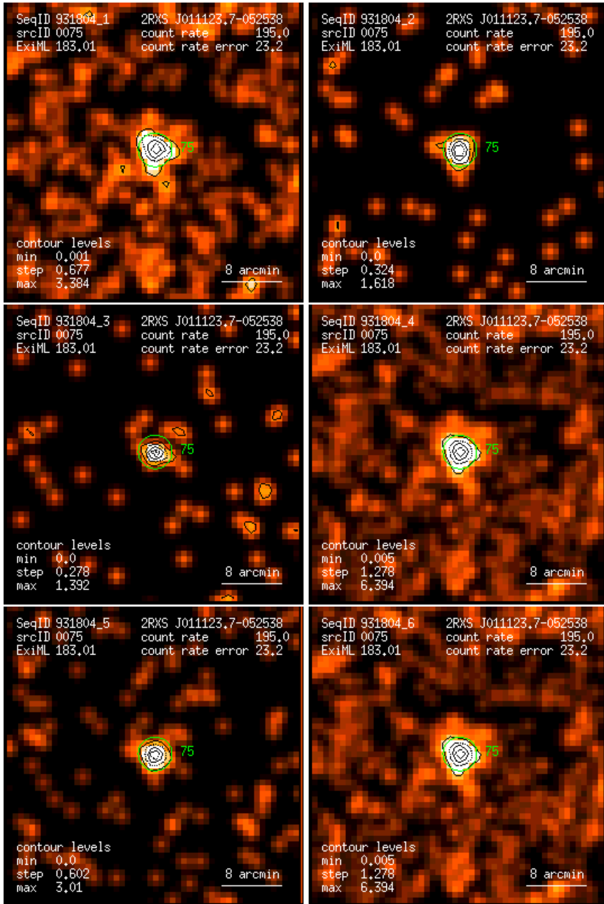
Figure 75: RASS 931804: detection 0075: band rate images, Gaussian filter: (1) PSPC channels 11 – 41, (2) 52 – 90, (3) 91 – 201, (4) 11 – 235, (5) 52 – 201, (6) 11 – 201. Broad band rates in counts/ks. Band rate contour levels in counts/ks/arcmin 2 .
