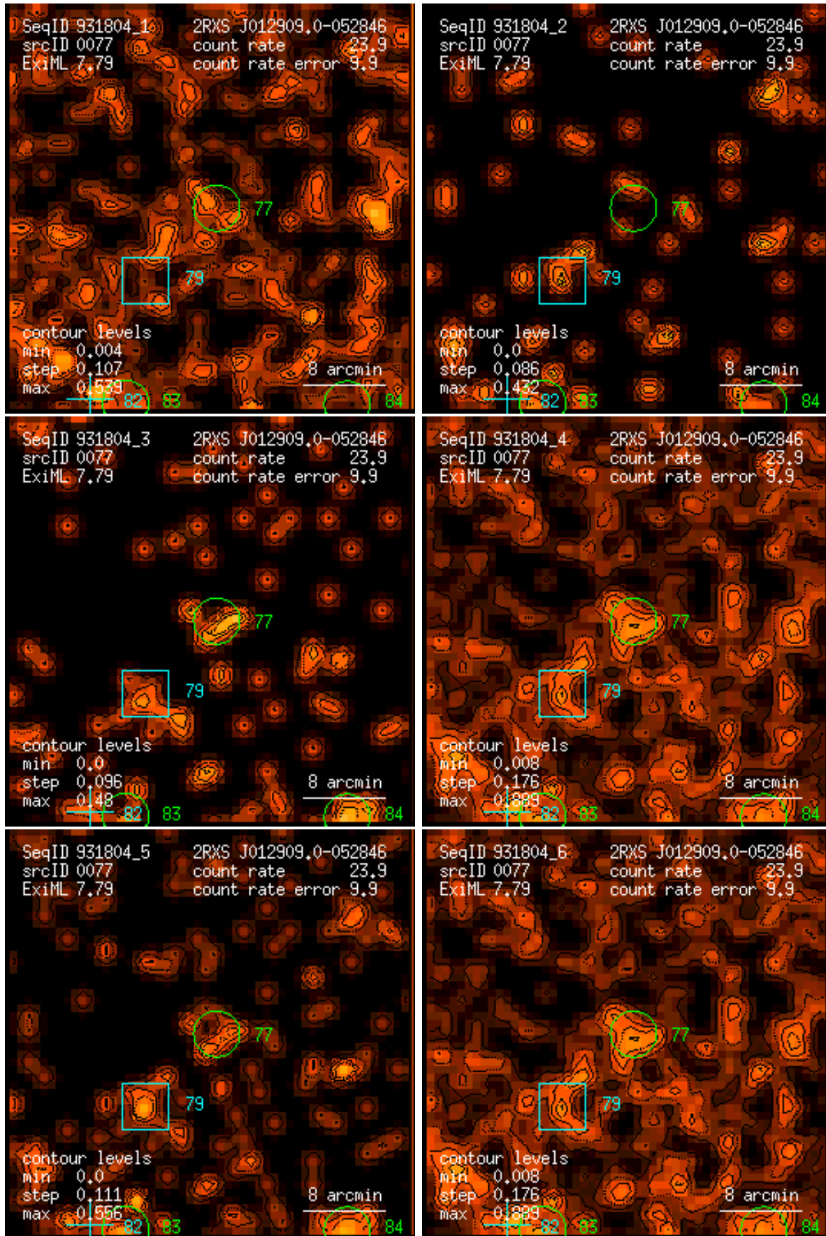
Figure 77: RASS 931804: detection 0077: band rate images, Gaussian filter: (1) PSPC channels 11 – 41, (2) 52 – 90, (3) 91 – 201, (4) 11 – 235, (5) 52 – 201, (6) 11 – 201. Broad band rates in counts/ks. Band rate contour levels in counts/ks/arcmin 2 .
