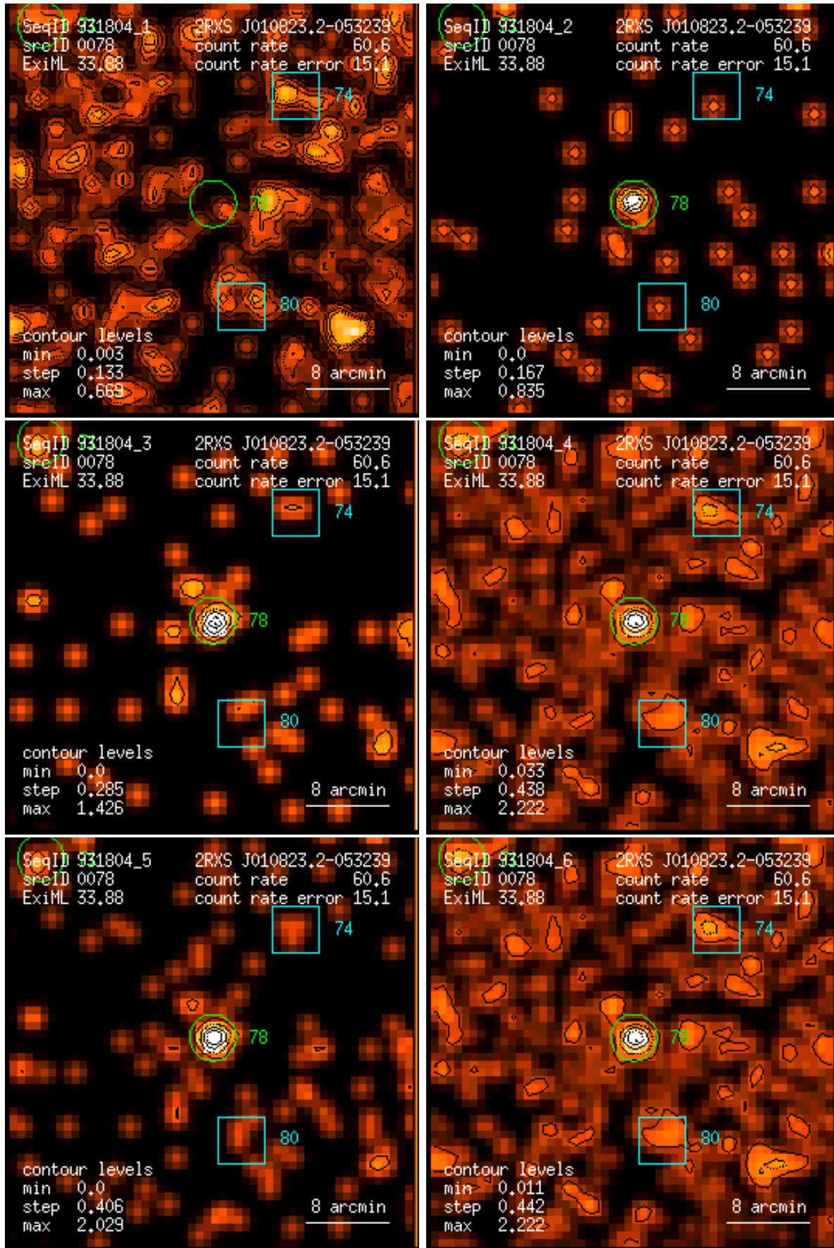
Figure 78: RASS 931804: detection 0078: band rate images, Gaussian filter: (1) PSPC channels 11 – 41, (2) 52 – 90, (3) 91 – 201, (4) 11 – 235, (5) 52 – 201, (6) 11 – 201. Broad band rates in counts/ks. Band rate contour levels in counts/ks/arcmin 2 .
