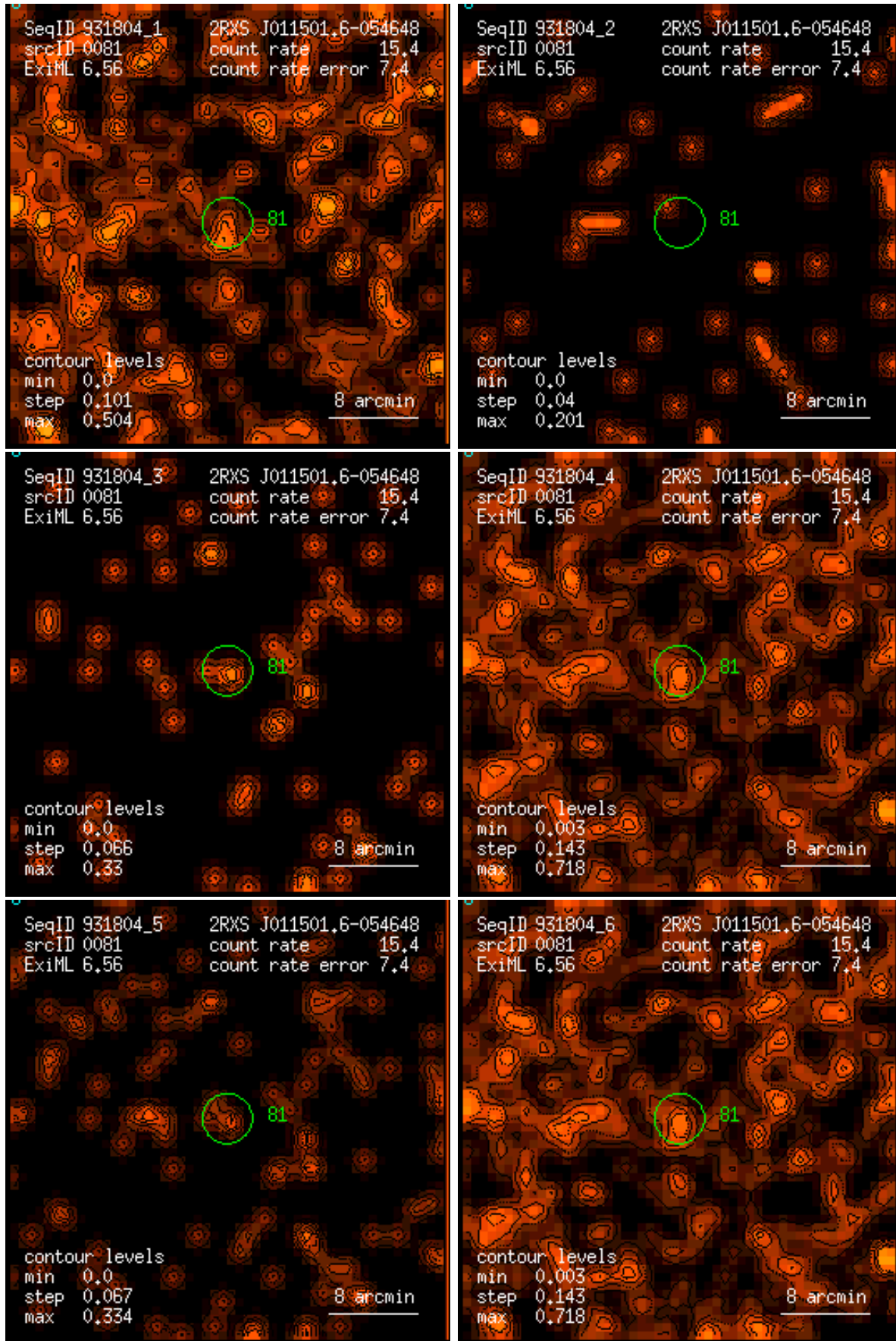
Figure 81: RASS 931804: detection 0081: band rate images, Gaussian filter: (1) PSPC channels 11 – 41, (2) 52 – 90, (3) 91 – 201, (4) 11 – 235, (5) 52 – 201, (6) 11 – 201. Broad band rates in counts/ks. Band rate contour levels in counts/ks/arcmin 2 .
