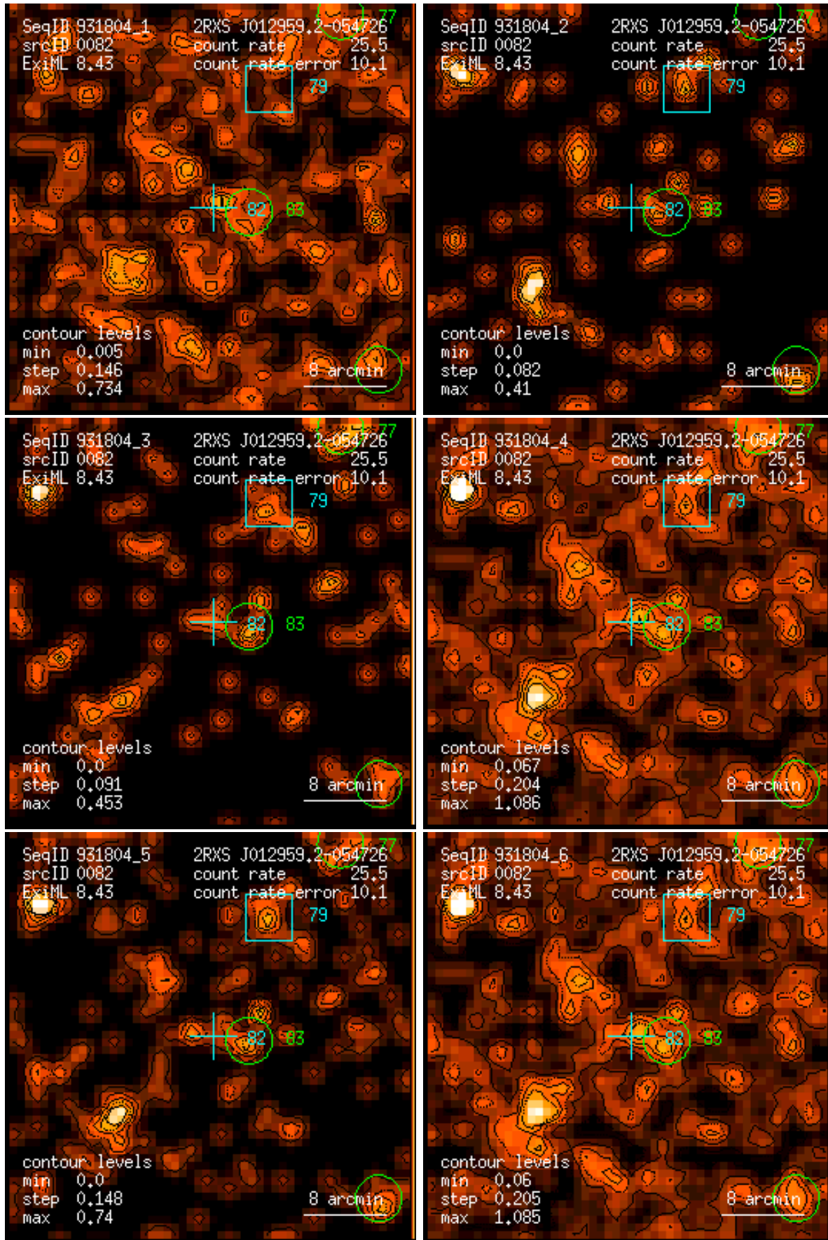
Figure 82: RASS 931804: detection 0082: band rate images, Gaussian filter: (1) PSPC channels 11 – 41, (2) 52 – 90, (3) 91 – 201, (4) 11 – 235, (5) 52 – 201, (6) 11 – 201. Broad band rates in counts/ks. Band rate contour levels in counts/ks/arcmin 2 .
