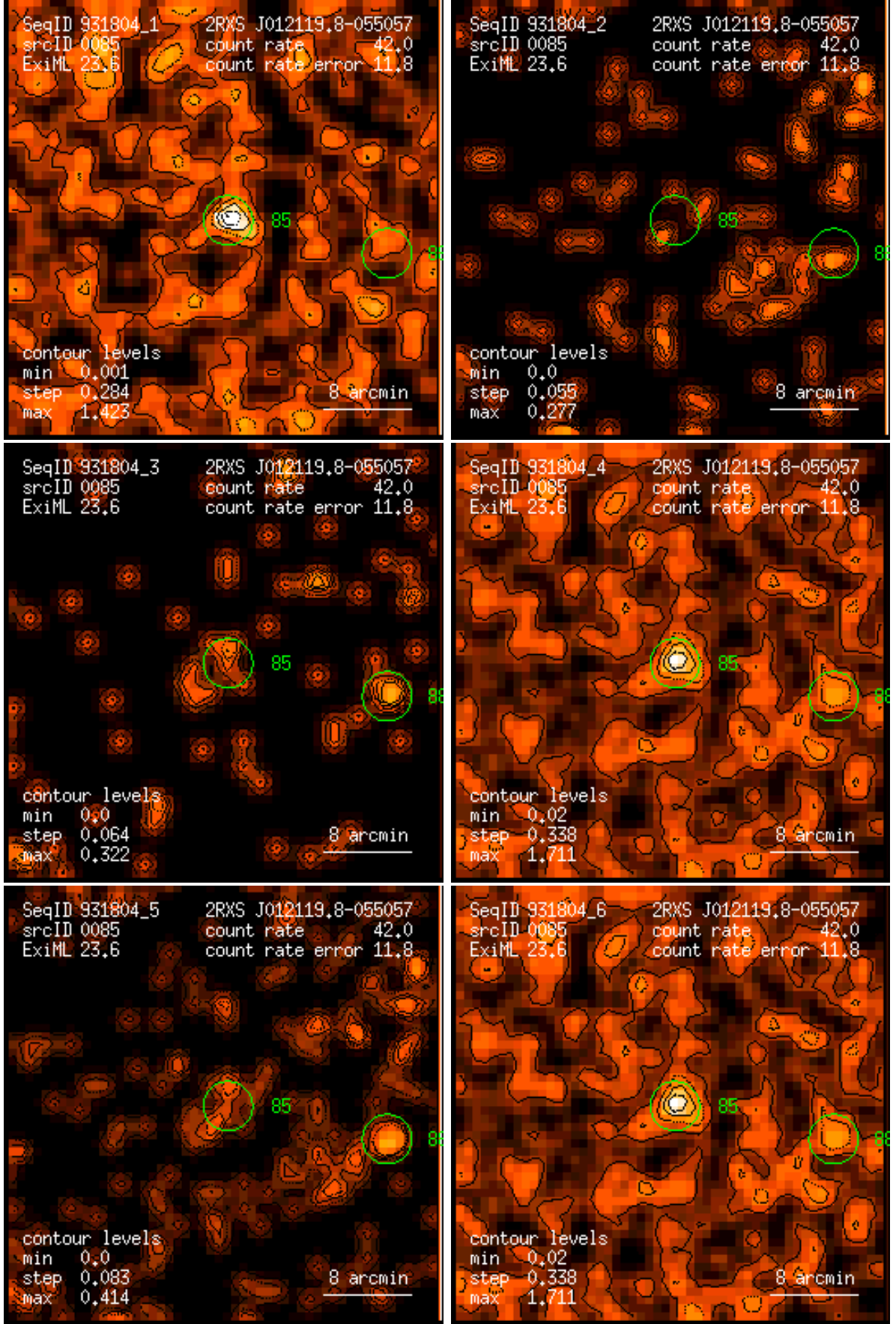
Figure 85: RASS 931804: detection 0085: band rate images, Gaussian filter: (1) PSPC channels 11 – 41, (2) 52 – 90, (3) 91 – 201, (4) 11 – 235, (5) 52 – 201, (6) 11 – 201. Broad band rates in counts/ks. Band rate contour levels in counts/ks/arcmin 2 .
