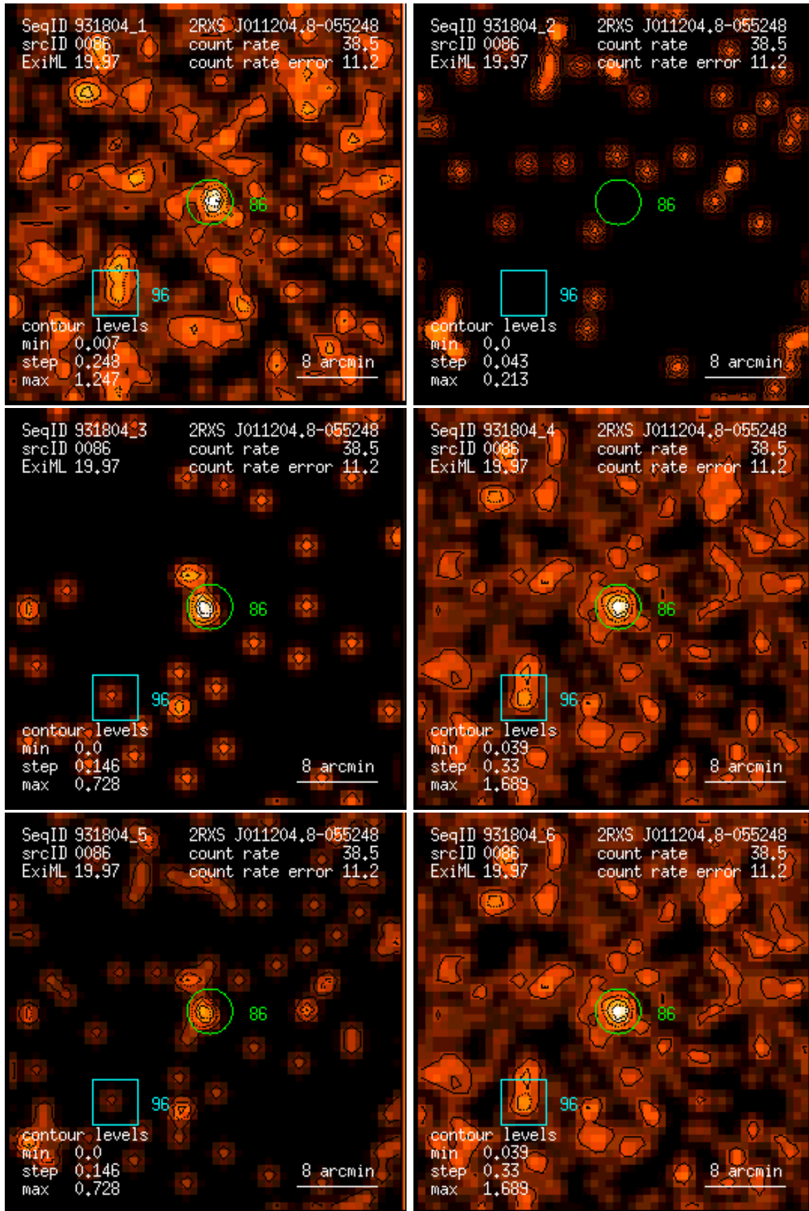
Figure 86: RASS 931804: detection 0086: band rate images, Gaussian filter: (1) PSPC channels 11 – 41, (2) 52 – 90, (3) 91 – 201, (4) 11 – 235, (5) 52 – 201, (6) 11 – 201. Broad band rates in counts/ks. Band rate contour levels in counts/ks/arcmin 2 .
