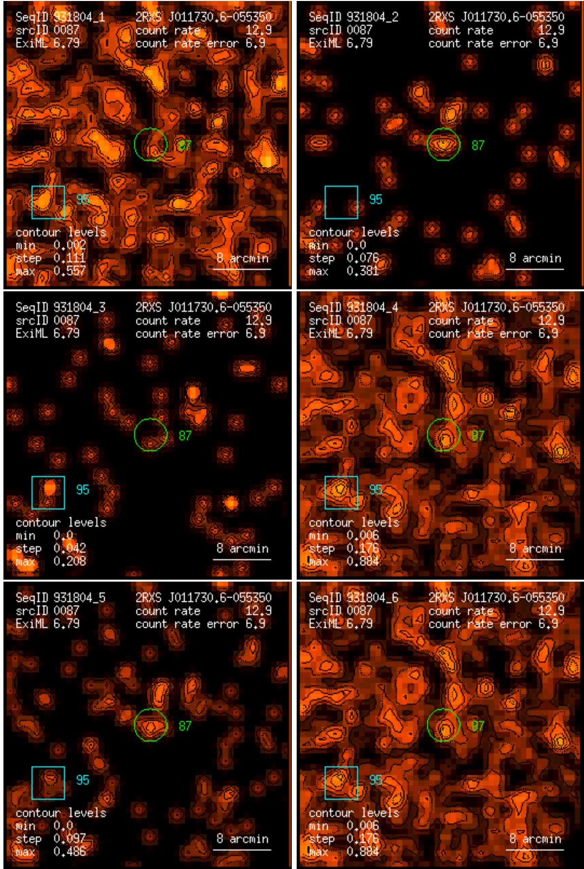
Figure 87: RASS 931804: detection 0087: band rate images, Gaussian filter: (1) PSPC channels 11 – 41, (2) 52 – 90, (3) 91 – 201, (4) 11 – 235, (5) 52 – 201, (6) 11 – 201. Broad band rates in counts/ks. Band rate contour levels in counts/ks/arcmin 2 .
