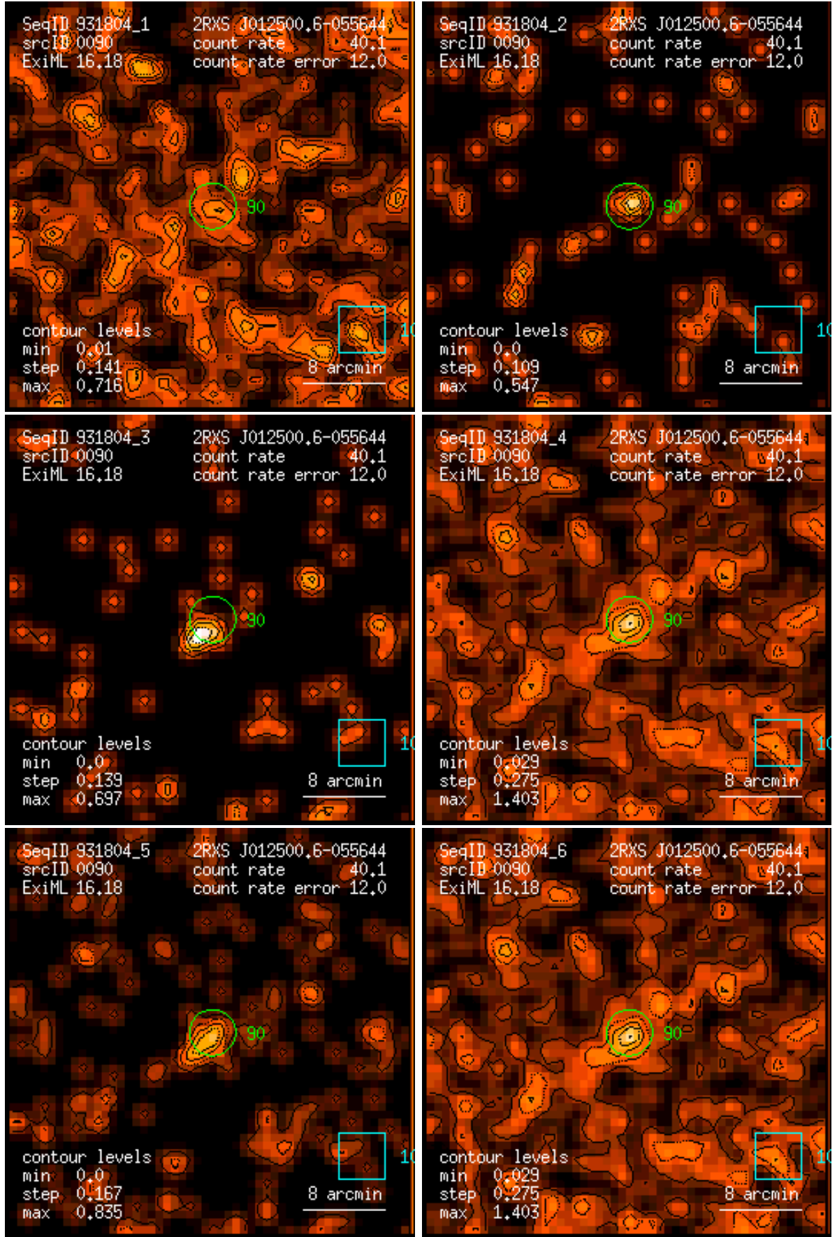
Figure 90: RASS 931804: detection 0090: band rate images, Gaussian filter: (1) PSPC channels 11 – 41, (2) 52 – 90, (3) 91 – 201, (4) 11 – 235, (5) 52 – 201, (6) 11 – 201. Broad band rates in counts/ks. Band rate contour levels in counts/ks/arcmin 2 .
