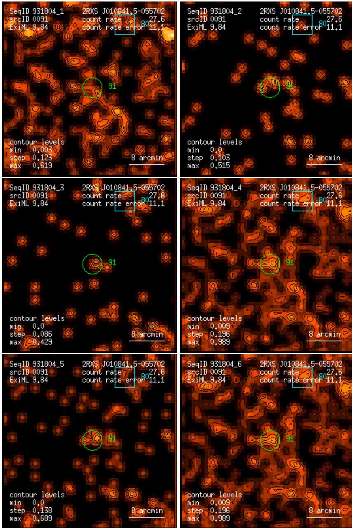
Figure 91: RASS 931804: detection 0091: band rate images, Gaussian filter: (1) PSPC channels 11 – 41, (2) 52 – 90, (3) 91 – 201, (4) 11 – 235, (5) 52 – 201, (6) 11 – 201. Broad band rates in counts/ks. Band rate contour levels in counts/ks/arcmin 2 .
