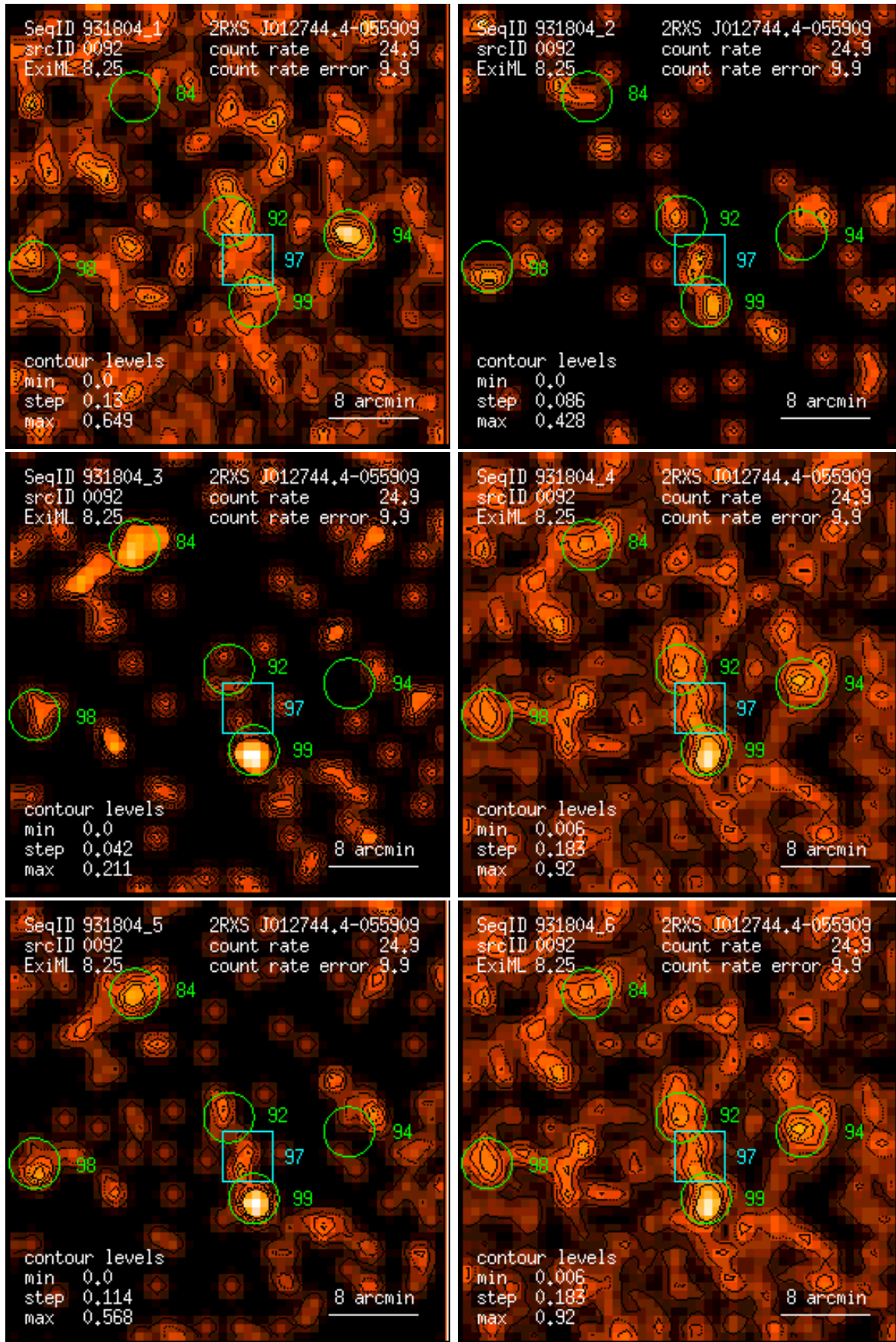
Figure 92: RASS 931804: detection 0092: band rate images, Gaussian filter: (1) PSPC channels 11 – 41, (2) 52 – 90, (3) 91 – 201, (4) 11 – 235, (5) 52 – 201, (6) 11 – 201. Broad band rates in counts/ks. Band rate contour levels in counts/ks/arcmin 2 .
