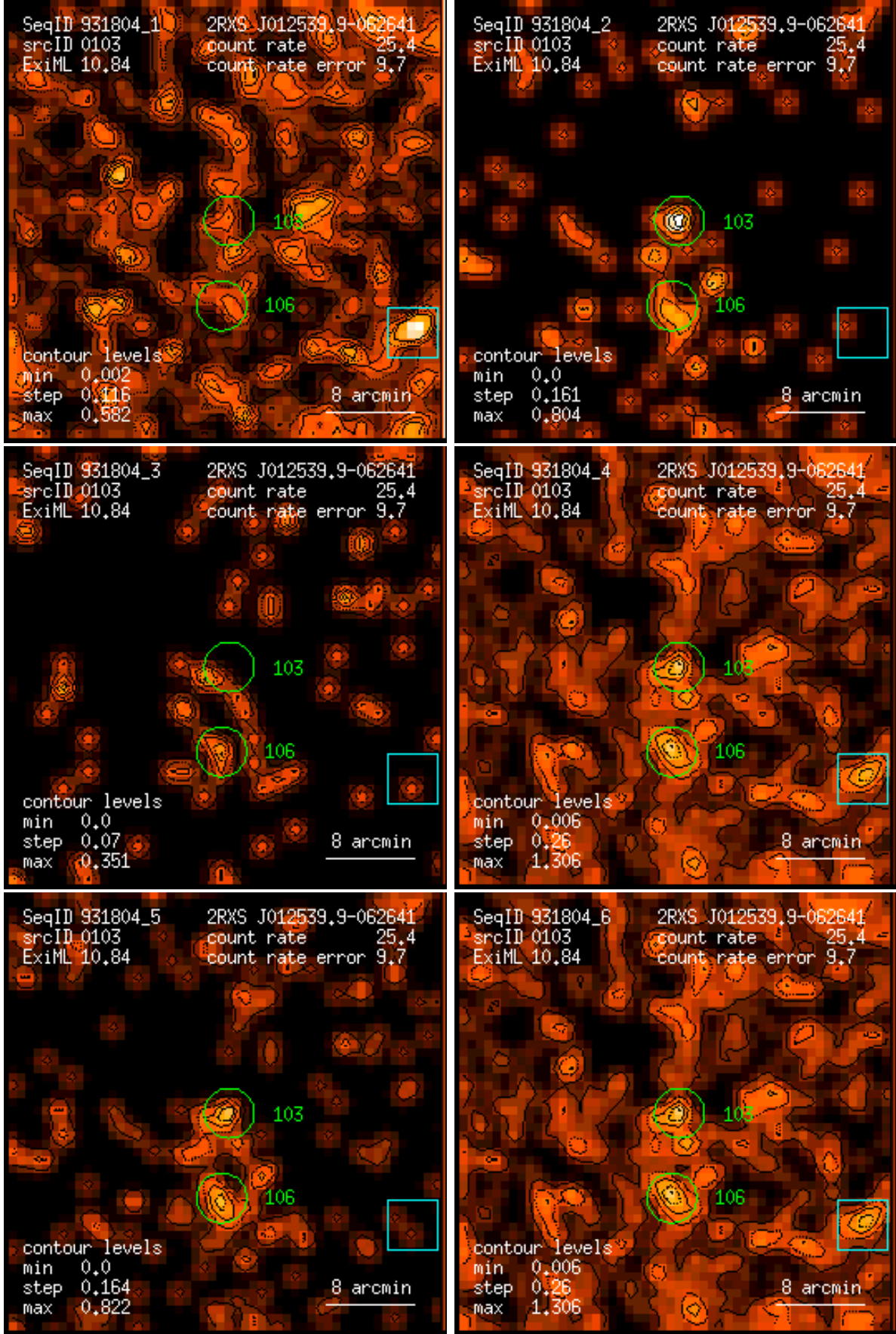
Figure 103: RASS 931804: detection 0103: band rate images, Gaussian filter: (1) PSPC channels 11 – 41, (2) 52 – 90, (3) 91 – 201, (4) 11 – 235, (5) 52 – 201, (6) 11 – 201. Broad band rates in counts/ks. Band rate contour levels in counts/ks/arcmin 2 .
