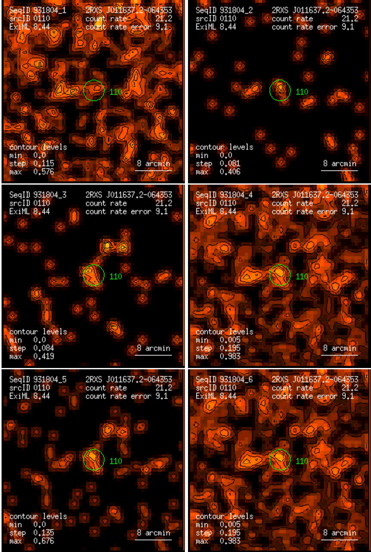
Figure 110: RASS 931804: detection 0110: band rate images, Gaussian filter: (1) PSPP channels 11 – 41, (2) 52 – 90, (3) 91 – 201, (4) 11 – 235, (5) 52 – 201, (6) 11 – 201. Broad band rates in counts/ks. Band rate contour levels in counts/ks/arcmin 2 .
