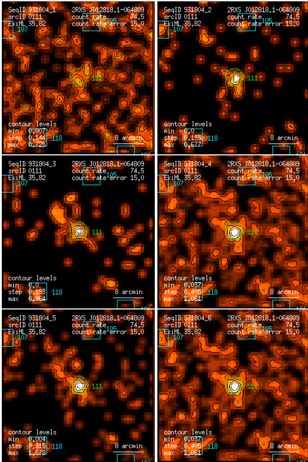
Figure 111: RASS 931804: detection 0111: band rate images, Gaussian filter: (1) PSPC channels 11 – 41, (2) 52 – 90, (3) 91 – 201, (4) 11 – 235, (5) 52 – 201, (6) 11 – 201. Broad band rates in counts/ks. Band rate contour levels in counts/ks/arcmin 2 .
