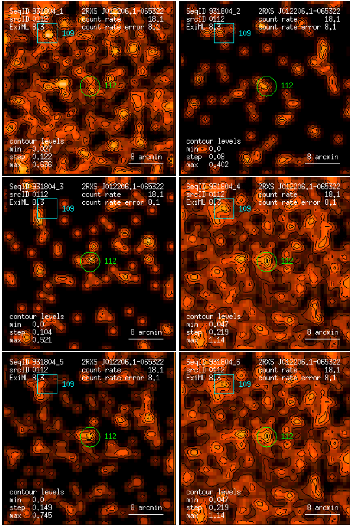
Figure 112: RASS 931804: detection 0112: band rate images, Gaussian filter: (1) PSPC channels 11 – 41, (2) 52 – 90, (3) 91 – 201, (4) 11 – 235, (5) 52 – 201, (6) 11 – 201. Broad band rates in counts/ks. Band rate contour levels in counts/ks/arcmin 2 .
