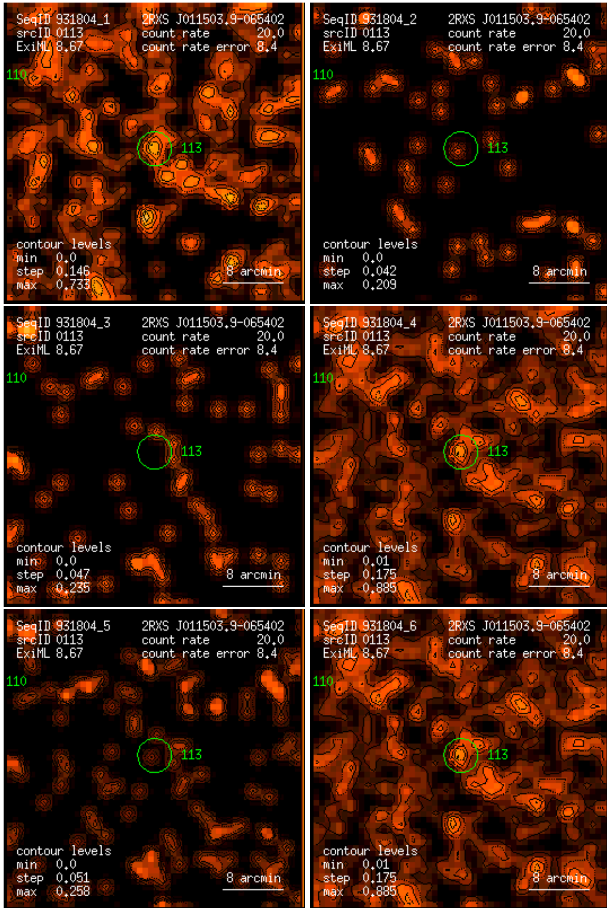
Figure 113: RASS 931804: detection 0113: band rate images, Gaussian filter: (1) PSPC channels 11 – 41, (2) 52 – 90, (3) 91 – 201, (4) 11 – 235, (5) 52 – 201, (6) 11 – 201. Broad band rates in counts/ks. Band rate contour levels in counts/ks/arcmin 2 .
