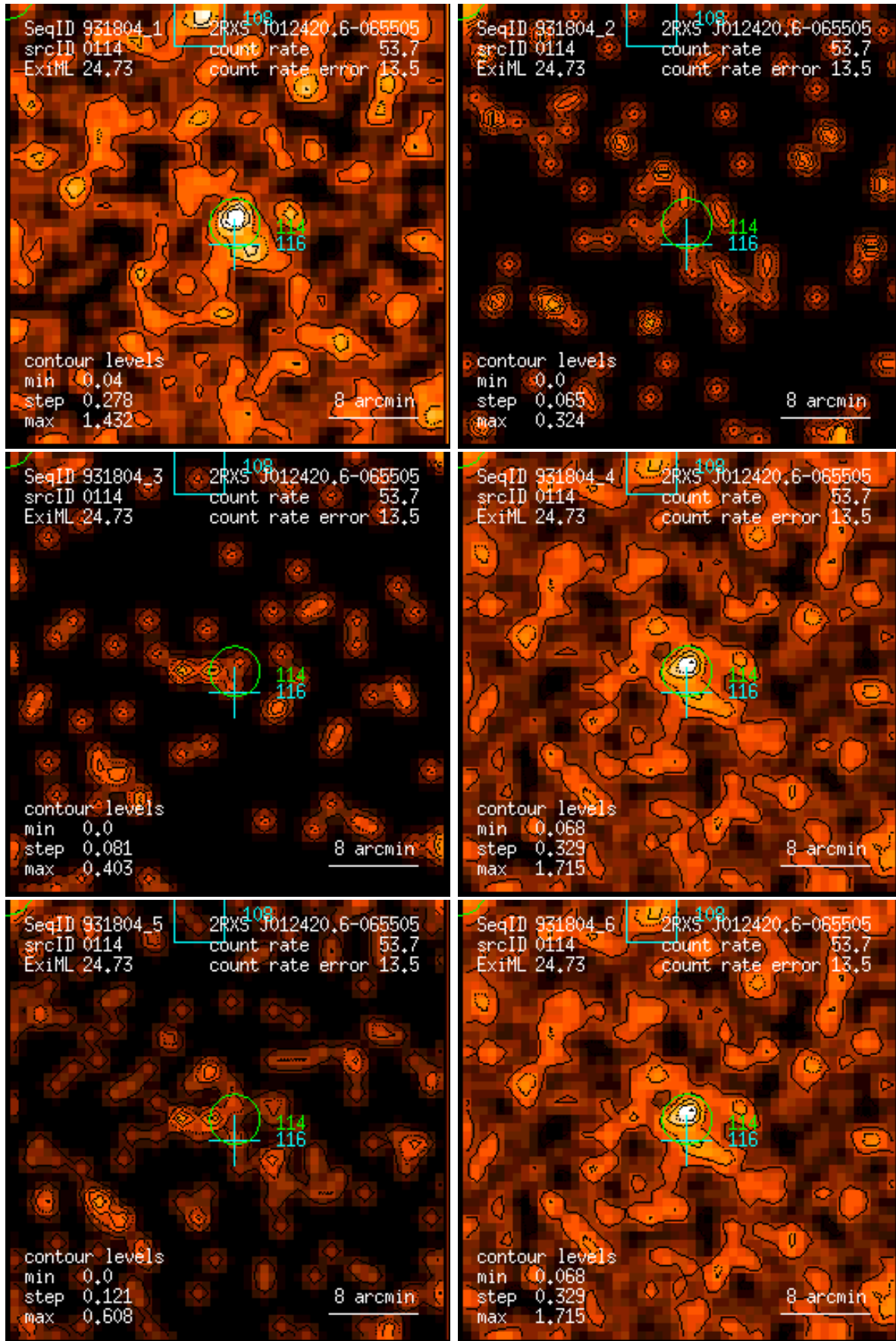
Figure 114: RASS 931804: detection 0114: band rate images, Gaussian filter: (1) PSPC channels 11 – 41, (2) 52 – 90, (3) 91 – 201, (4) 11 – 235, (5) 52 – 201, (6) 11 – 201. Broad band rates in counts/ks. Band rate contour levels in counts/ks/arcmin 2 .
