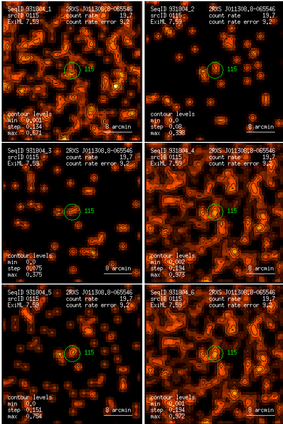
Figure 115: RASS 931804: detection 0115: band rate images, Gaussian filter: (1) PSPC channels 11 – 41, (2) 52 – 90, (3) 91 – 201, (4) 11 – 235, (5) 52 – 201, (6) 11 – 201. Broad band rates in counts/ks. Band rate contour levels in counts/ks/arcmin 2 .
