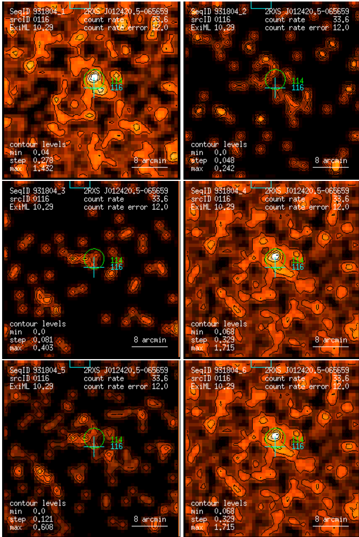
Figure 116: RASS 931804: detection 0116: band rate images, Gaussian filter: (1) PSPC channels 11 – 41, (2) 52 – 90, (3) 91 – 201, (4) 11 – 235, (5) 52 – 201, (6) 11 – 201. Broad band rates in counts/ks. Band rate contour levels in counts/ks/arcmin 2 .
