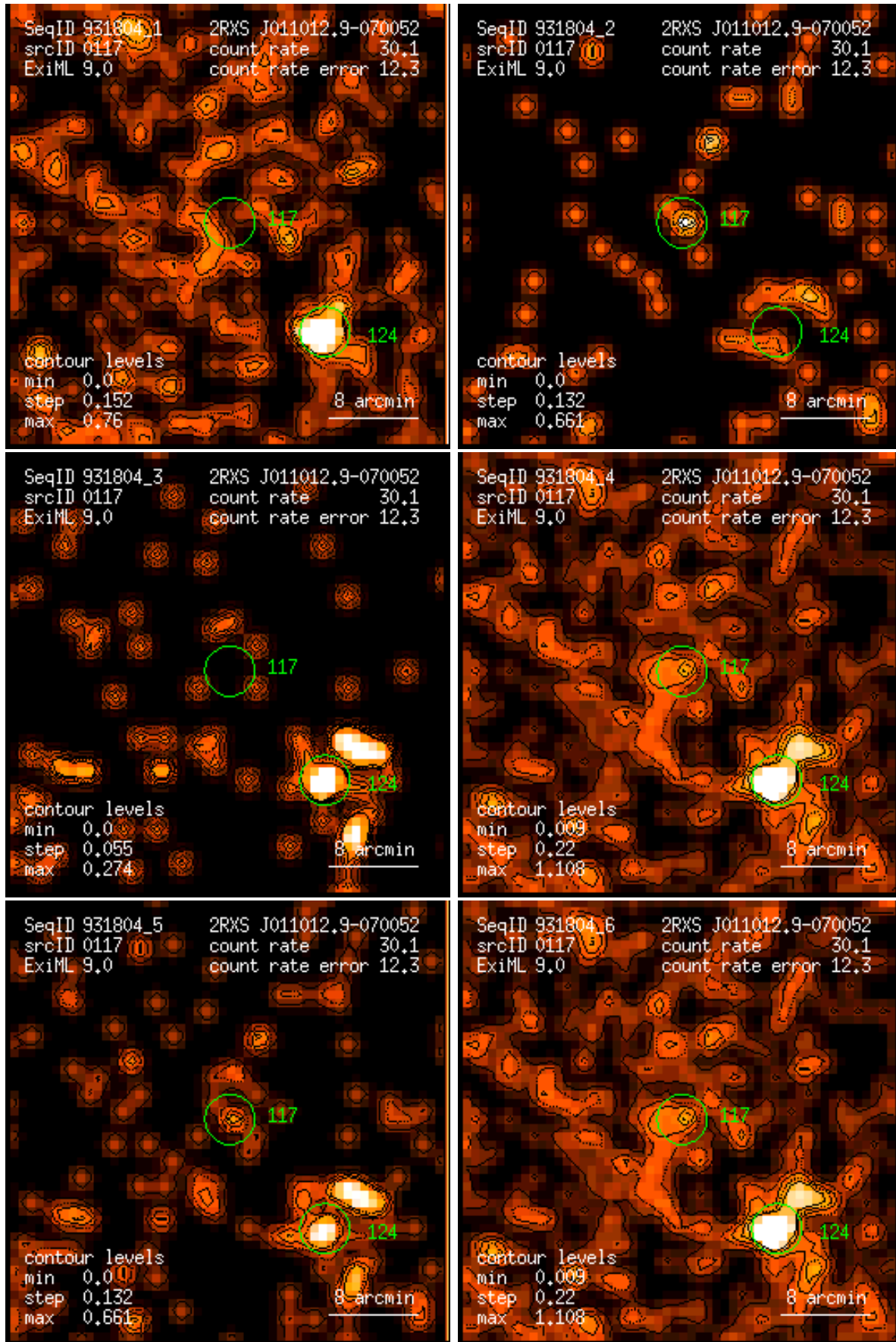
Figure 117: RASS 931804: detection 0117: band rate images, Gaussian filter: (1) PSPC channels 11 – 41, (2) 52 – 90, (3) 91 – 201, (4) 11 – 235, (5) 52 – 201, (6) 11 – 201. Broad band rates in counts/ks. Band rate contour levels in counts/ks/arcmin 2 .
