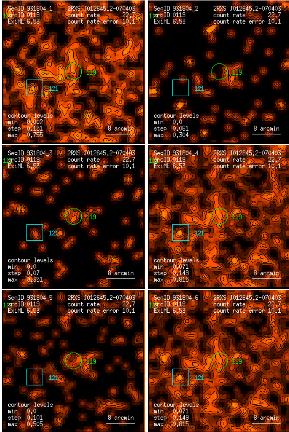
Figure 119: RASS 931804: detection 0119: band rate images, Gaussian filter: (1) PSPC channels 11 – 41, (2) 52 – 90, (3) 91 – 201, (4) 11 – 235, (5) 52 – 201, (6) 11 – 201. Broad band rates in counts/ks. Band rate contour levels in counts/ks/arcmin 2 .
