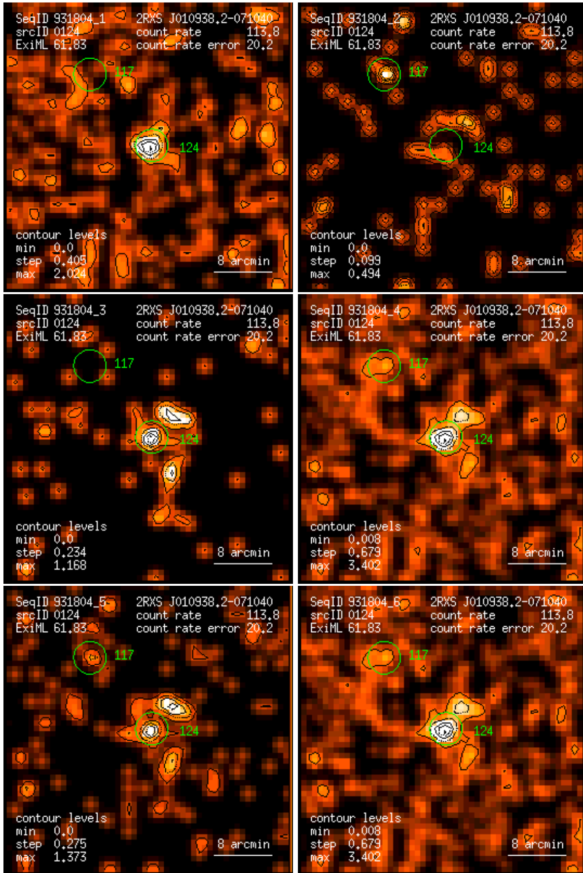
Figure 124: RASS 931804: detection 0124: band rate images, Gaussian filter: (1) PSPC channels 11 – 41, (2) 52 – 90, (3) 91 – 201, (4) 11 – 235, (5) 52 – 201, (6) 11 – 201. Broad band rates in counts/ks. Band rate contour levels in counts/ks/arcmin 2 .
