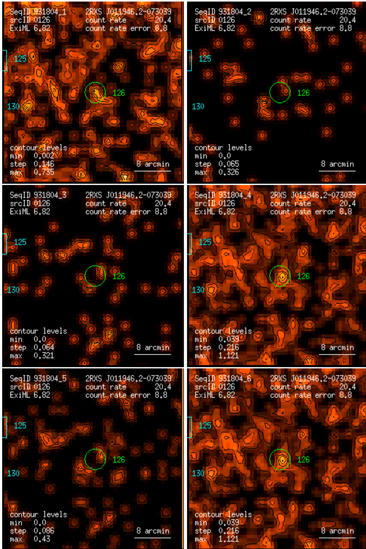
Figure 126: RASS 931804: detection 0126: band rate images, Gaussian filter: (1) PSPC channels 11 – 41, (2) 52 – 90, (3) 91 – 201, (4) 11 – 235, (5) 52 – 201, (6) 11 – 201. Broad band rates in counts/ks. Band rate contour levels in counts/ks/arcmin 2 .
