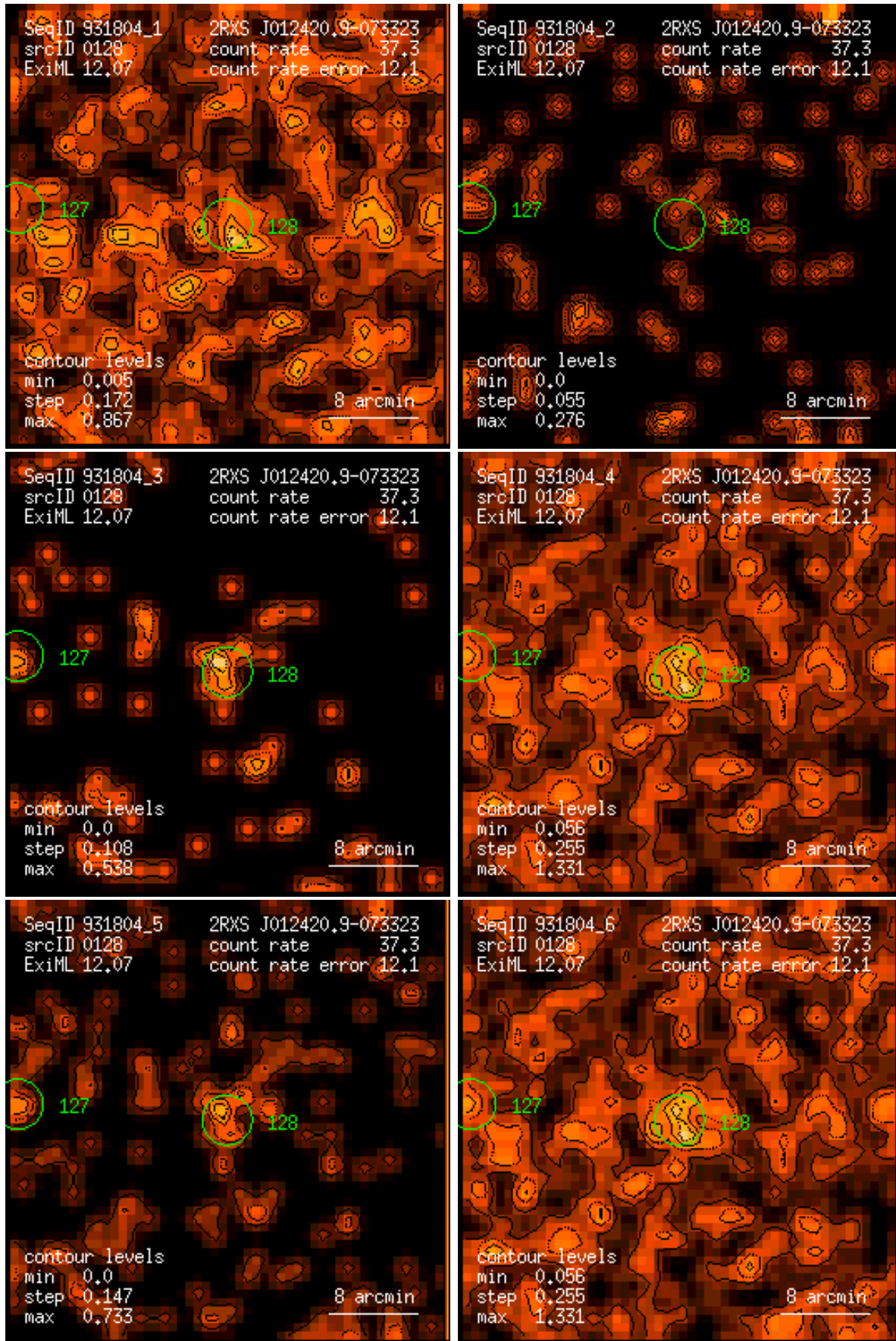
Figure 128: RASS 931804: detection 0128: band rate images, Gaussian filter: (1) PSPC channels 11 – 41, (2) 52 – 90, (3) 91 – 201, (4) 11 – 235, (5) 52 – 201, (6) 11 – 201. Broad band rates in counts/ks. Band rate contour levels in counts/ks/arcmin 2 .
