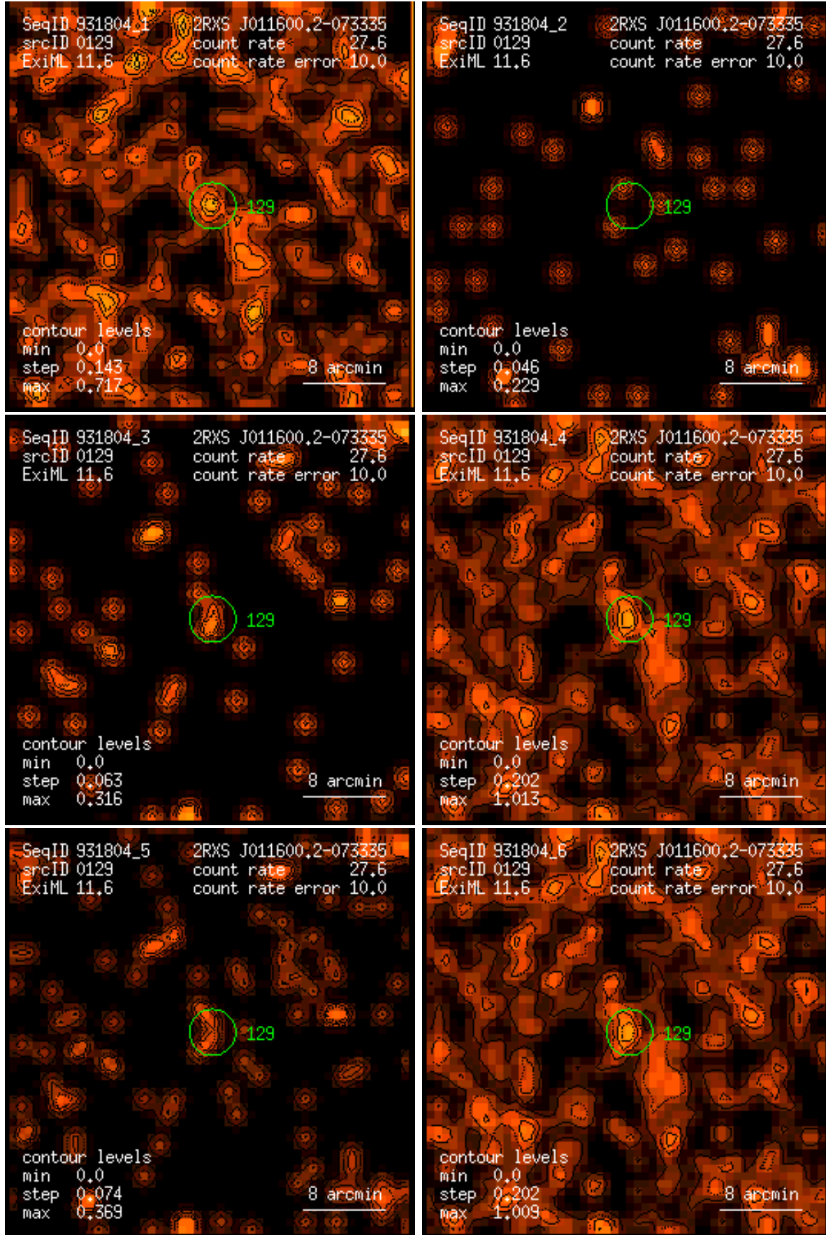
Figure 129: RASS 931804: detection 0129: band rate images, Gaussian filter: (1) PSPC channels 11 – 41, (2) 52 – 90, (3) 91 – 201, (4) 11 – 235, (5) 52 – 201, (6) 11 – 201. Broad band rates in counts/ks. Band rate contour levels in counts/ks/arcmin 2 .
