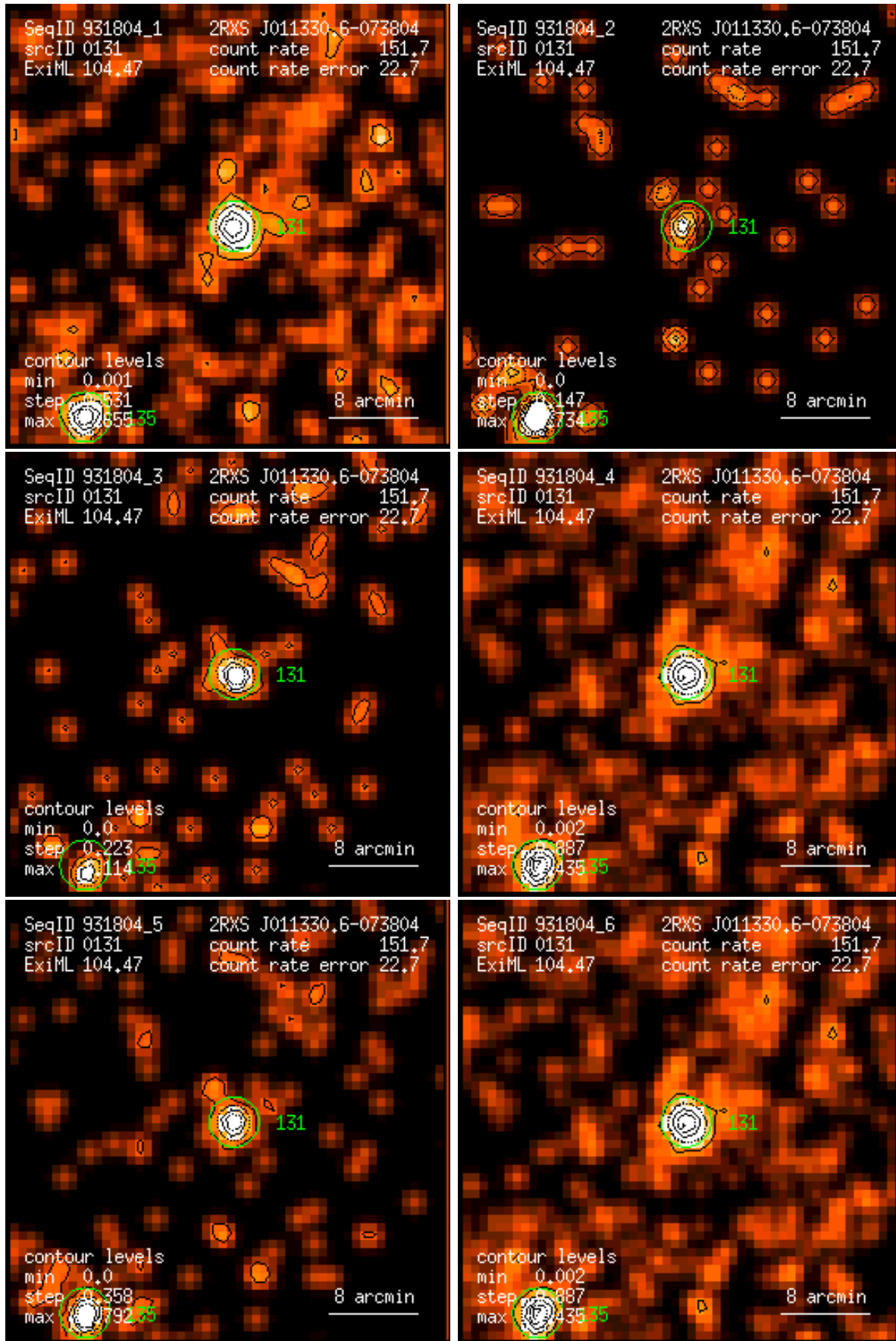
Figure 131: RASS 931804: detection 0131: band rate images, Gaussian filter: (1) PSPC channels 11 – 41, (2) 52 – 90, (3) 91 – 201, (4) 11 – 235, (5) 52 – 201, (6) 11 – 201. Broad band rates in counts/ks. Band rate contour levels in counts/ks/arcmin 2 .
