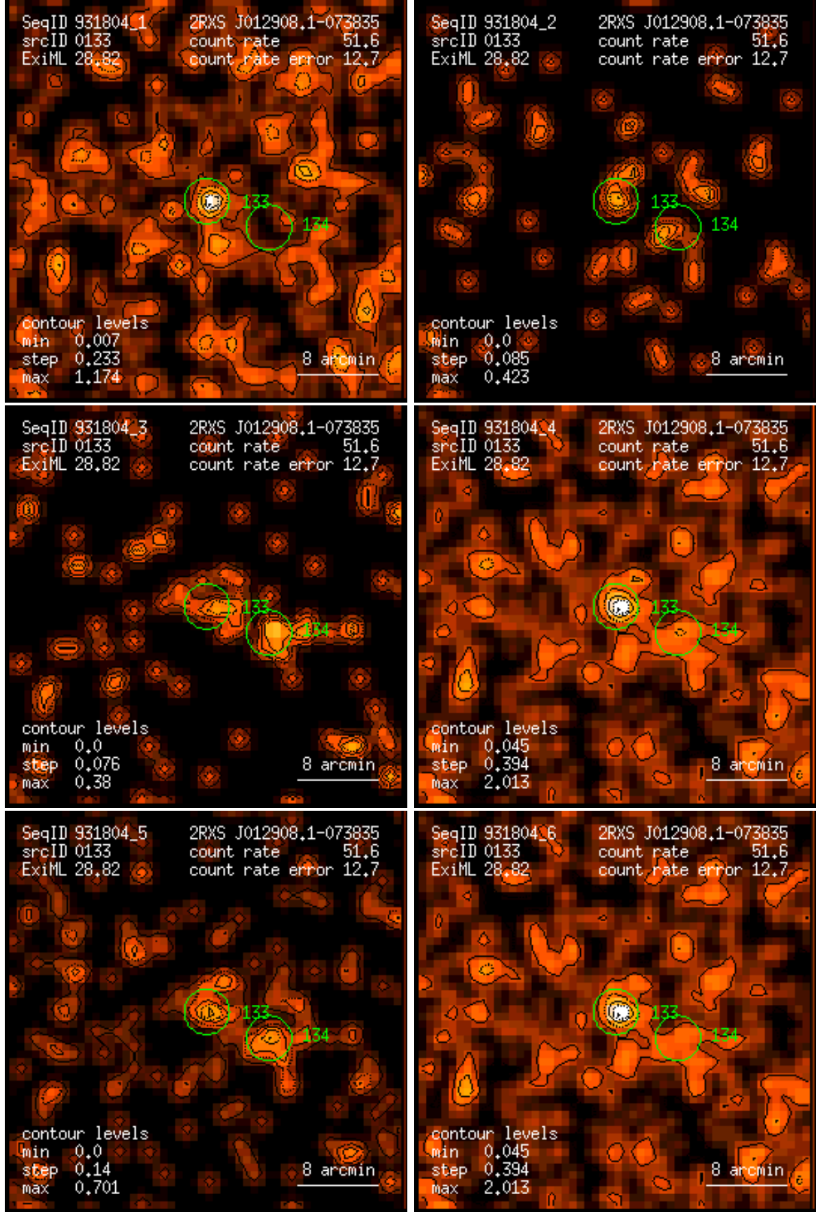
Figure 133: RASS 931804: detection 0133: band rate images, Gaussian filter: (1) PSPC channels 11 – 41, (2) 52 – 90, (3) 91 – 201, (4) 11 – 235, (5) 52 – 201, (6) 11 – 201. Broad band rates in counts/ks. Band rate contour levels in counts/ks/arcmin 2 .
