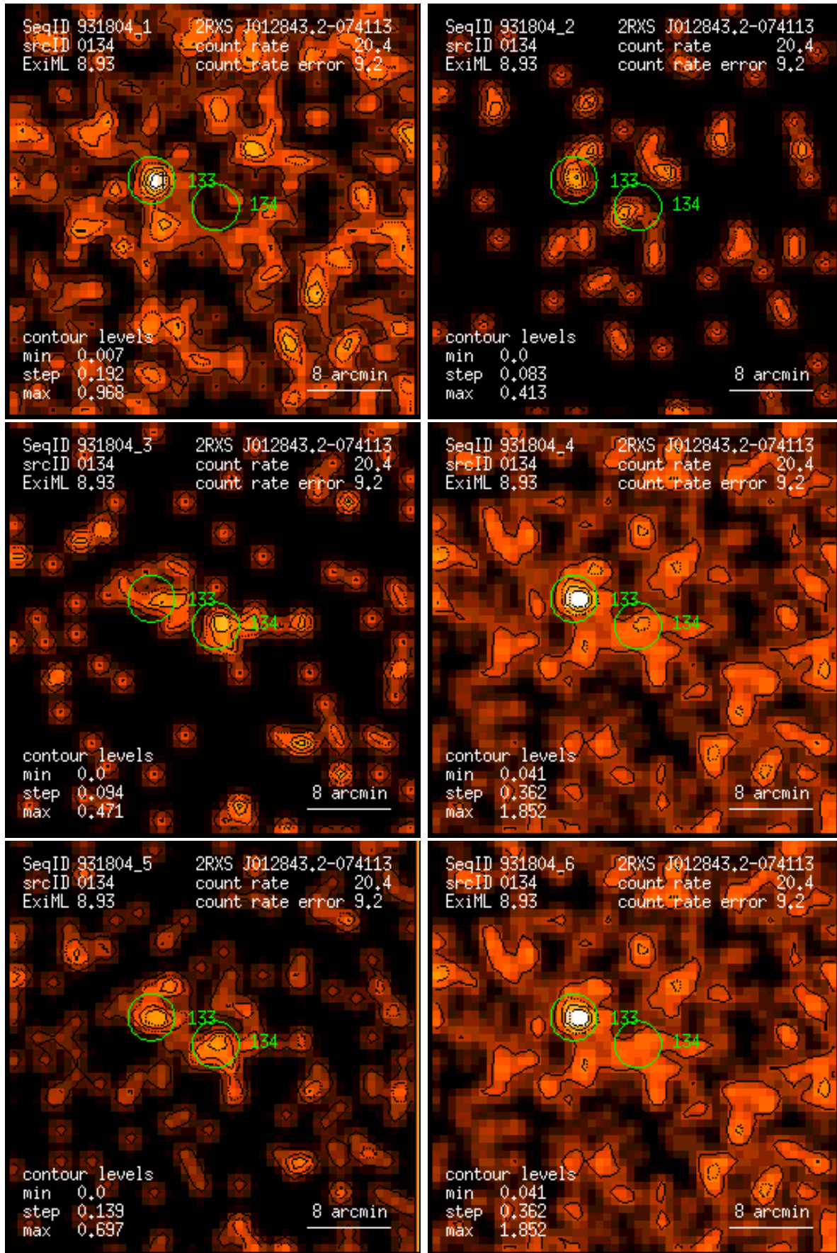
Figure 134: RASS 931804: detection 0134: band rate images, Gaussian filter: (1) PSPC channels 11 – 41, (2) 52 – 90, (3) 91 – 201, (4) 11 – 235, (5) 52 – 201, (6) 11 – 201. Broad band rates in counts/ks. Band rate contour levels in counts/ks/arcmin 2 .
