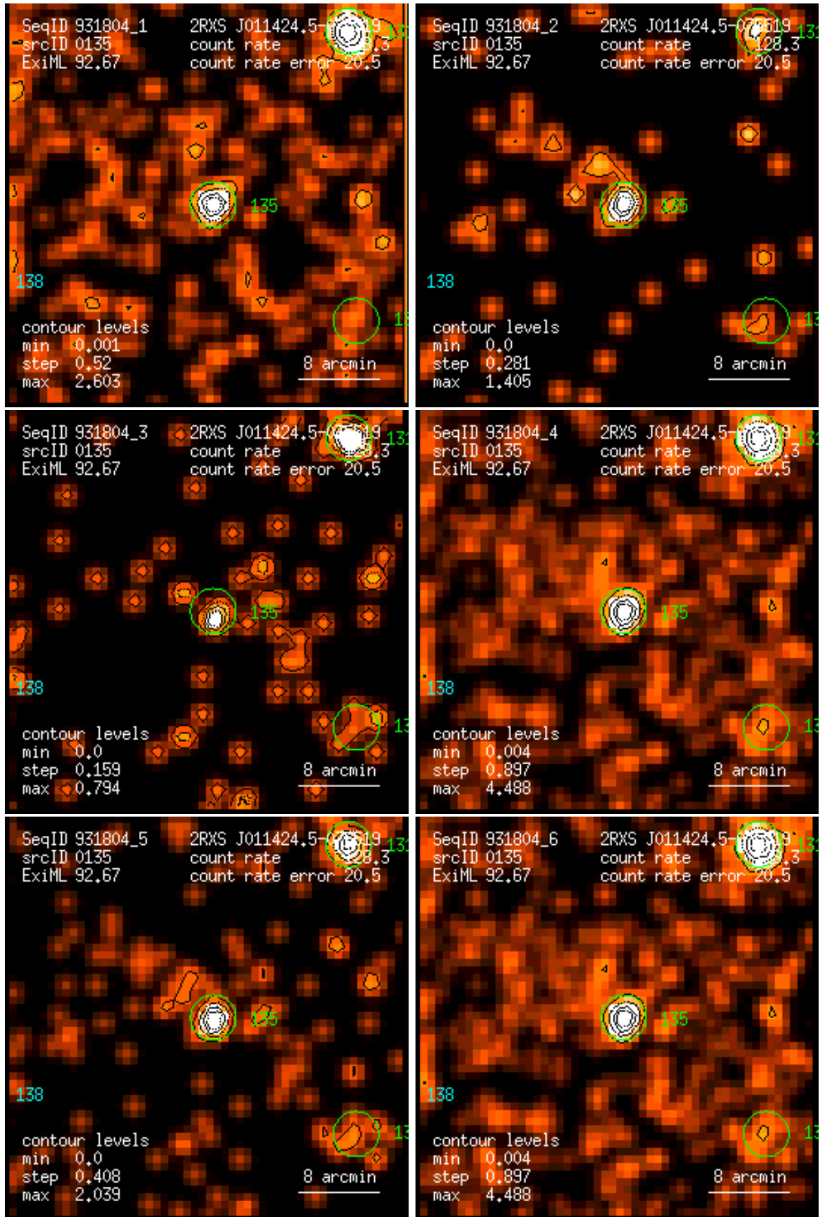
Figure 135: RASS 931804: detection 0135: band rate images, Gaussian filter: (1) PSPC channels 11 – 41, (2) 52 – 90, (3) 91 – 201, (4) 11 – 235, (5) 52 – 201, (6) 11 – 201. Broad band rates in counts/ks. Band rate contour levels in counts/ks/arcmin 2 .
