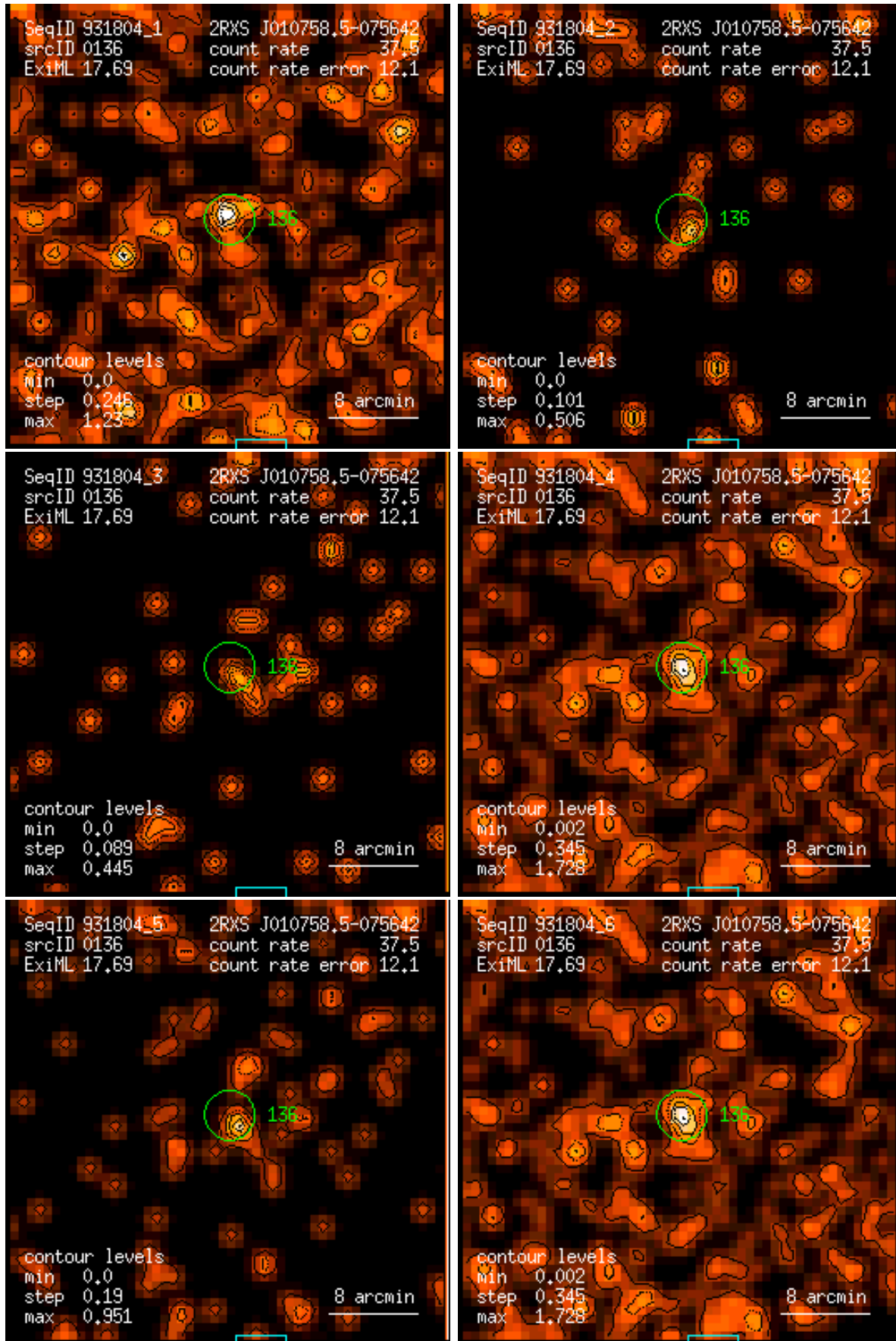
Figure 136: RASS 931804: detection 0136: band rate images, Gaussian filter: (1) PSPC channels 11 – 41, (2) 52 – 90, (3) 91 – 201, (4) 11 – 235, (5) 52 – 201, (6) 11 – 201. Broad band rates in counts/ks. Band rate contour levels in counts/ks/arcmin 2 .
