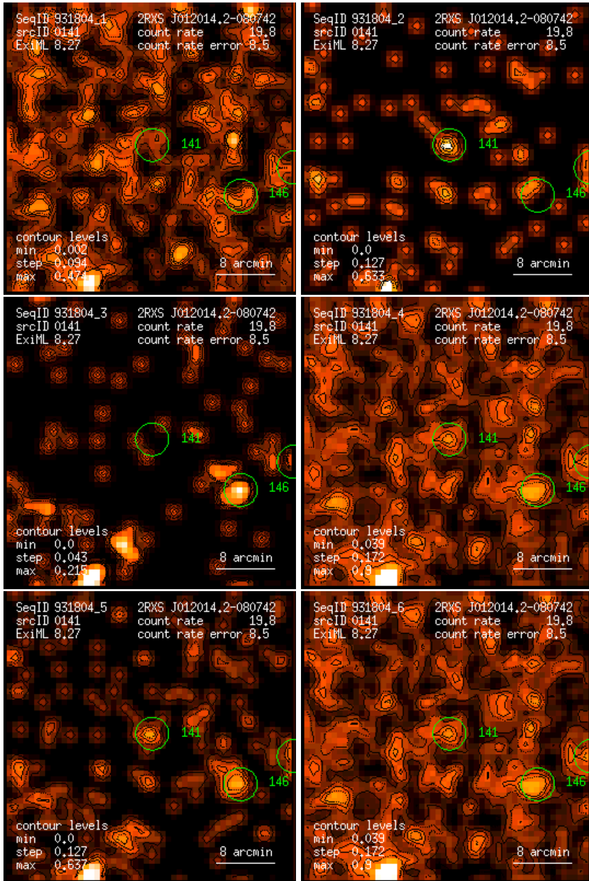
Figure 141: RASS 931804: detection 0141: band rate images, Gaussian filter: (1) PSPC channels 11 – 41, (2) 52 – 90, (3) 91 – 201, (4) 11 – 235, (5) 52 – 201, (6) 11 – 201. Broad band rates in counts/ks. Band rate contour levels in counts/ks/arcmin 2 .
