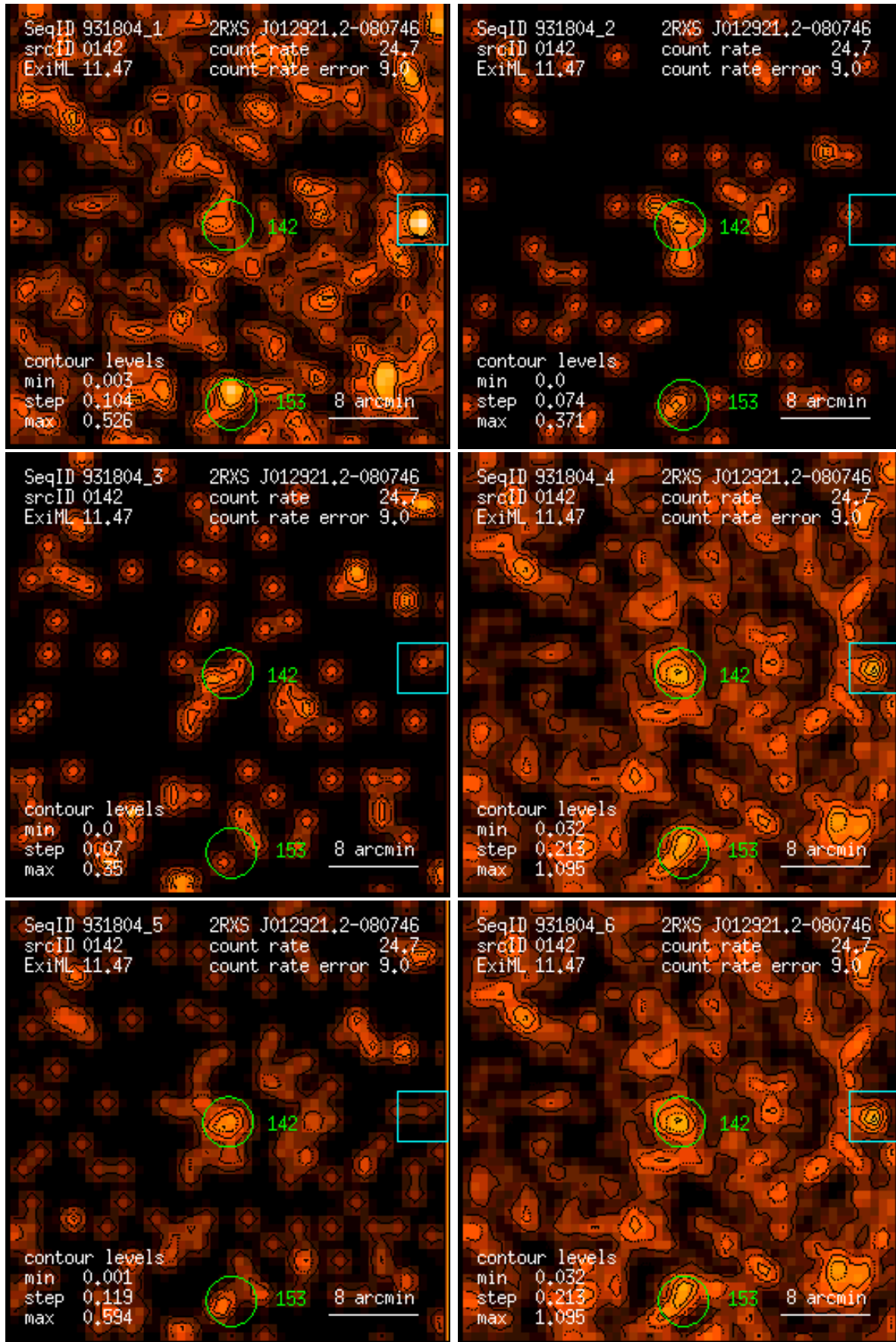
Figure 142: RASS 931804: detection 0142: band rate images, Gaussian filter: (1) PSPC channels 11 – 41, (2) 52 – 90, (3) 91 – 201, (4) 11 – 235, (5) 52 – 201, (6) 11 – 201. Broad band rates in counts/ks. Band rate contour levels in counts/ks/arcmin 2 .
