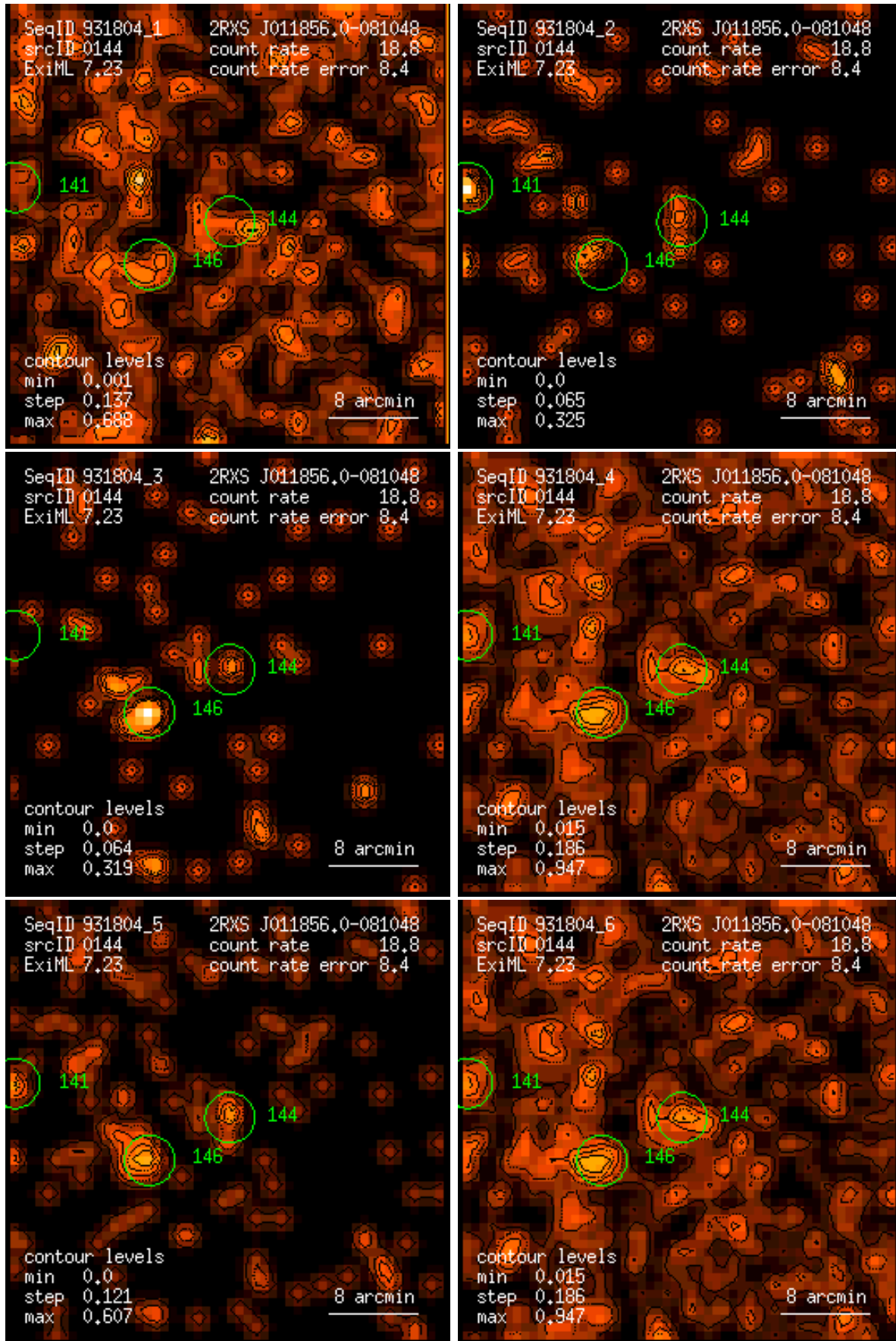
Figure 144: RASS 931804: detection 0144: band rate images, Gaussian filter: (1) PSPC channels 11 – 41, (2) 52 – 90, (3) 91 – 201, (4) 11 – 235, (5) 52 – 201, (6) 11 – 201. Broad band rates in counts/ks. Band rate contour levels in counts/ks/arcmin 2 .
