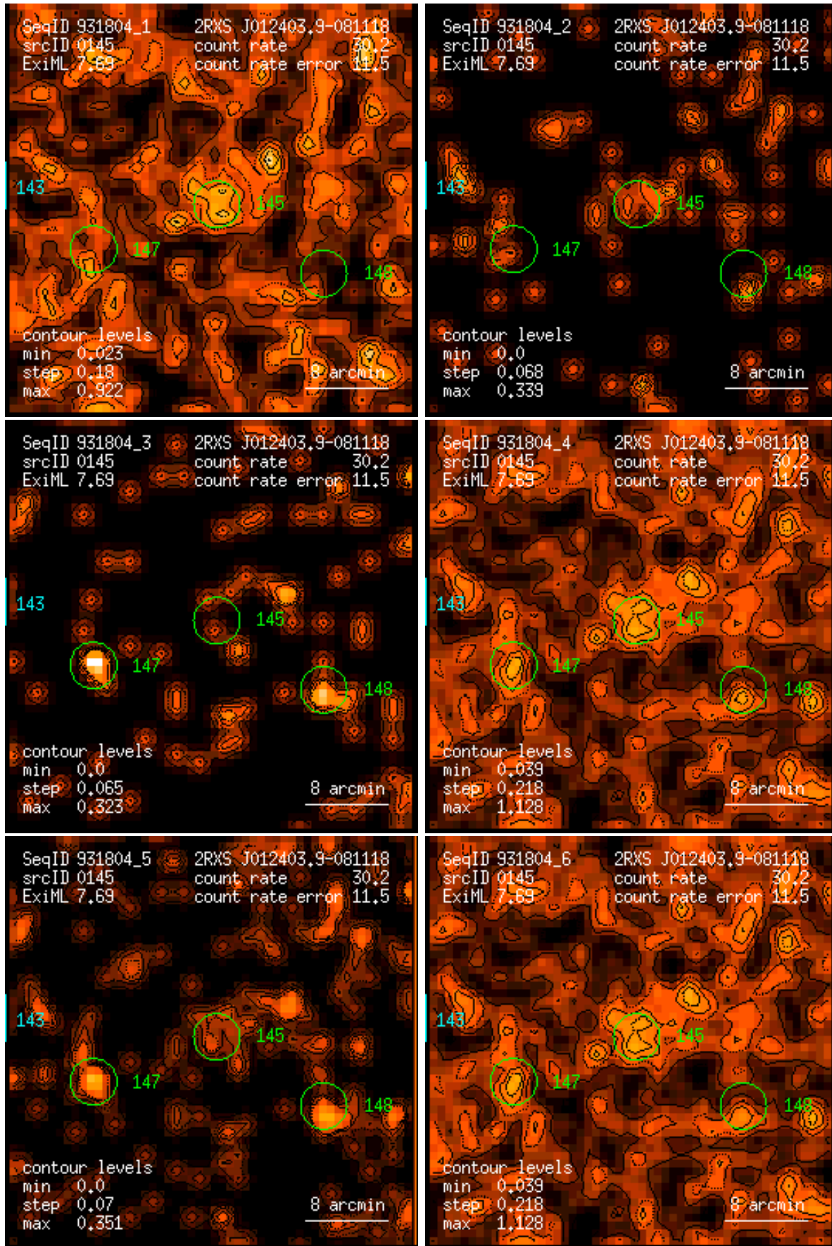
Figure 145: RASS 931804: detection 0145: band rate images, Gaussian filter: (1) PSPC channels 11 – 41, (2) 52 – 90, (3) 91 – 201, (4) 11 – 235, (5) 52 – 201, (6) 11 – 201. Broad band rates in counts/ks. Band rate contour levels in counts/ks/arcmin 2 .
