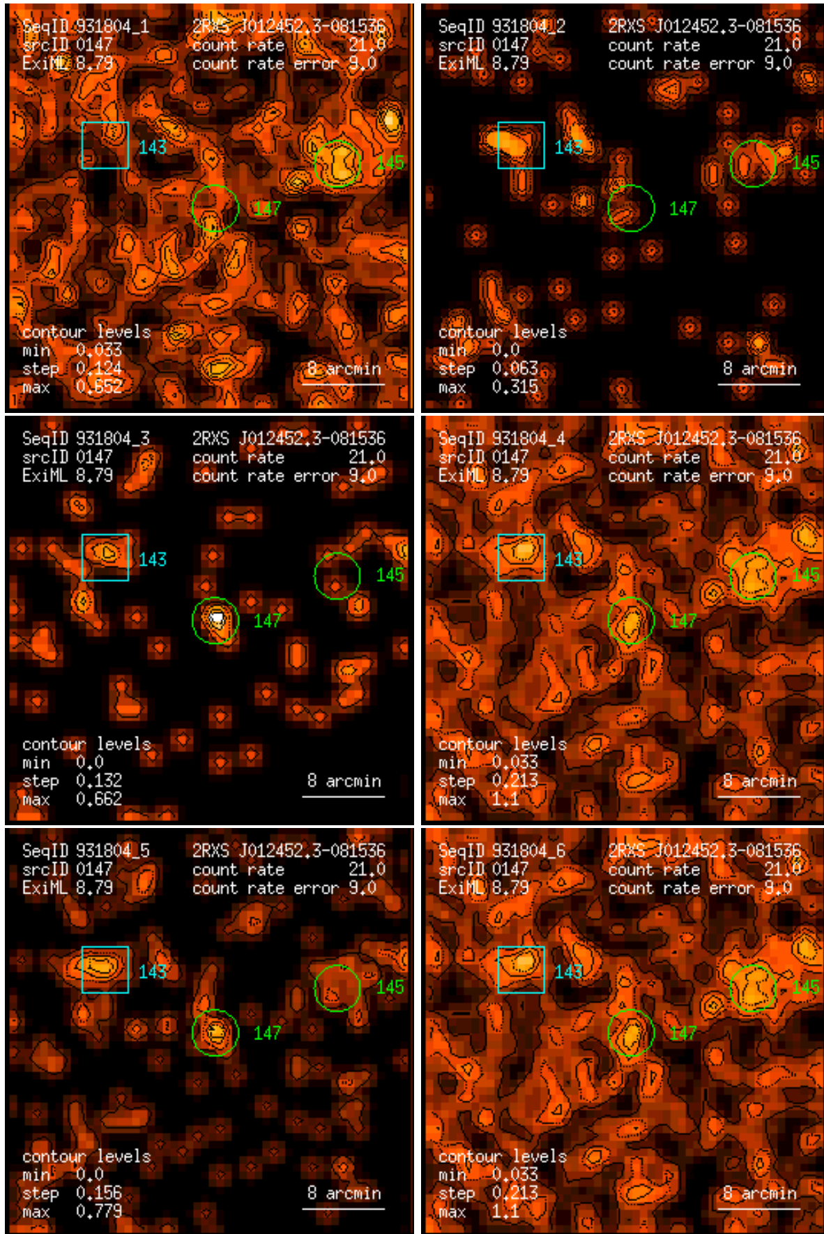
Figure 147: RASS 931804: detection 0147: band rate images, Gaussian filter: (1) PSPC channels 11 – 41, (2) 52 – 90, (3) 91 – 201, (4) 11 – 235, (5) 52 – 201, (6) 11 – 201. Broad band rates in counts/ks. Band rate contour levels in counts/ks/arcmin 2 .
