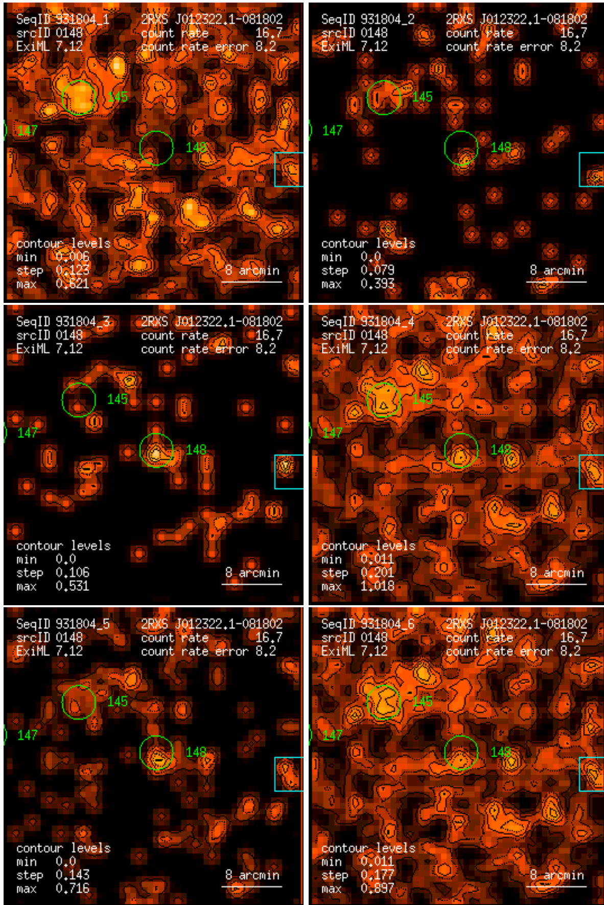
Figure 148: RASS 931804: detection 0148: band rate images, Gaussian filter: (1) PSPC channels 11 – 41, (2) 52 – 90, (3) 91 – 201, (4) 11 – 235, (5) 52 – 201, (6) 11 – 201. Broad band rates in counts/ks. Band rate contour levels in counts/ks/arcmin 2 .
