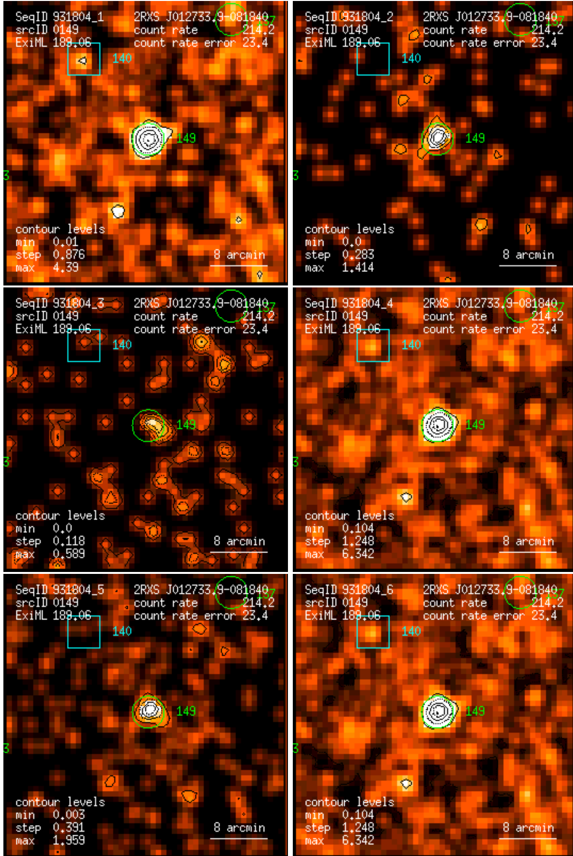
Figure 149: RASS 931804: detection 0149: band rate images, Gaussian filter: (1) PSPC channels 11 – 41, (2) 52 – 90, (3) 91 – 201, (4) 11 – 235, (5) 52 – 201, (6) 11 – 201. Broad band rates in counts/ks. Band rate contour levels in counts/ks/arcmin 2 .
