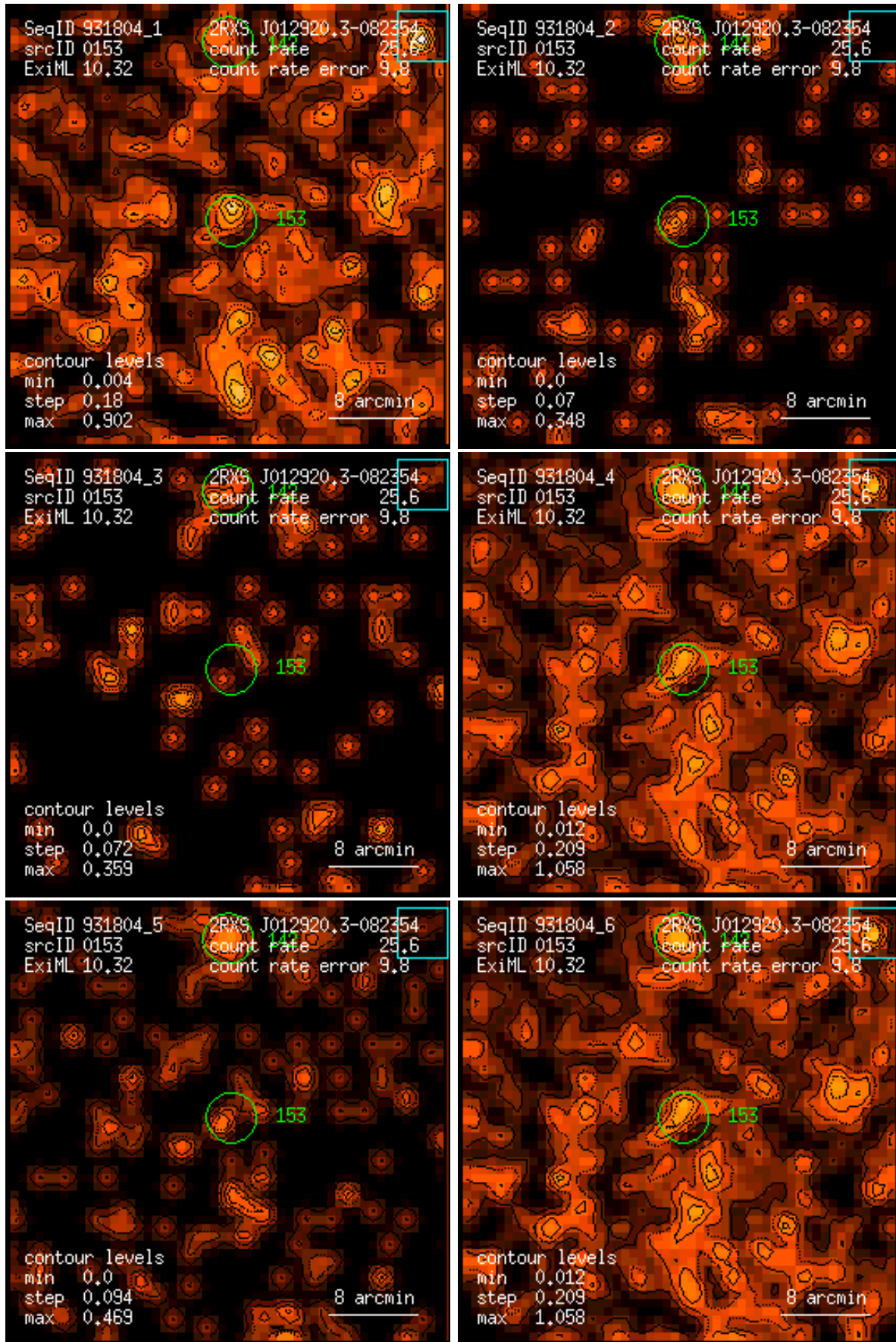
Figure 153: RASS 931804: detection 0153: band rate images, Gaussian filter: (1) PSPC channels 11 – 41, (2) 52 – 90, (3) 91 – 201, (4) 11 – 235, (5) 52 – 201, (6) 11 – 201. Broad band rates in counts/ks. Band rate contour levels in counts/ks/arcmin 2 .
