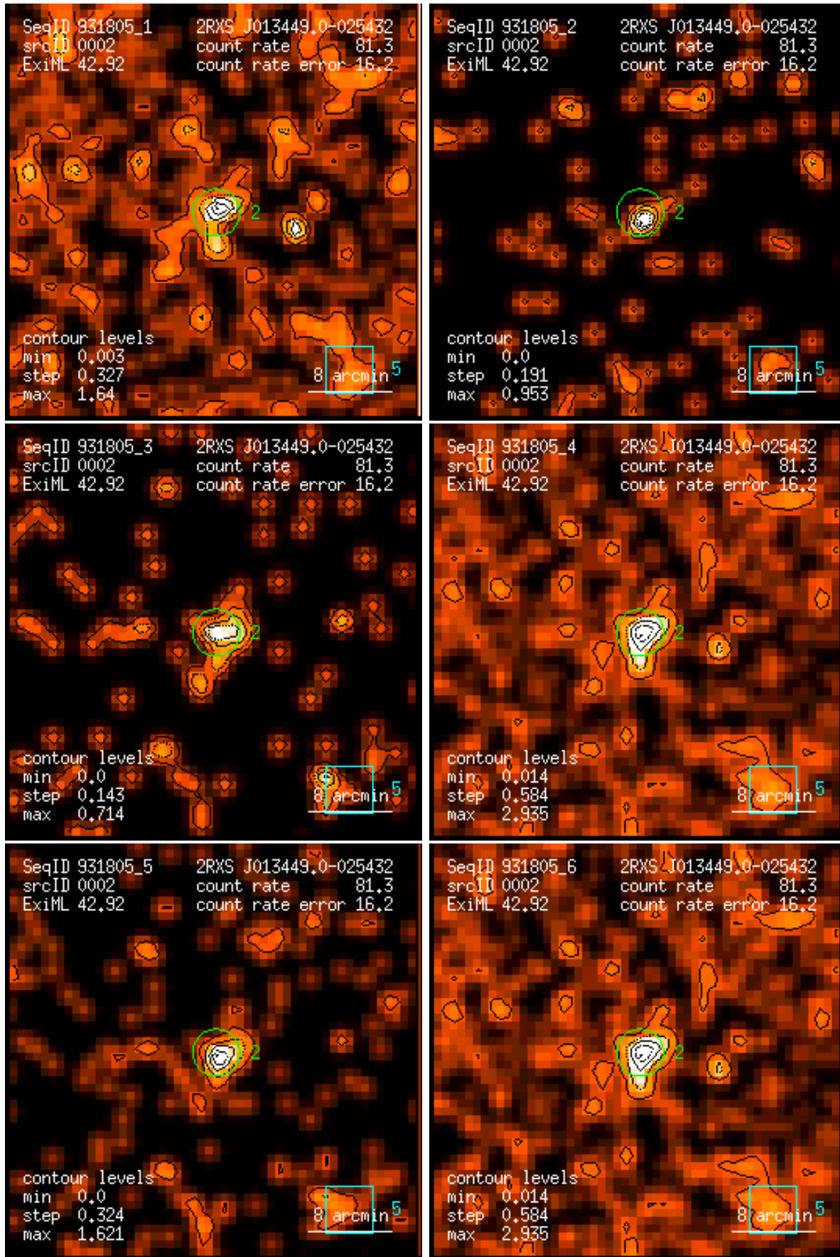
Figure 2: RASS 931805: detection 0002: band rate images, Gaussian filter: (1) PSPC channels 11 – 41, (2) 52 – 90, (3) 91 – 201, (4) 11 – 235, (5) 52 – 201, (6) 11 – 201. Broad band rates in counts/ks. Band rate contour levels in counts/ks/arcmin 2 .
