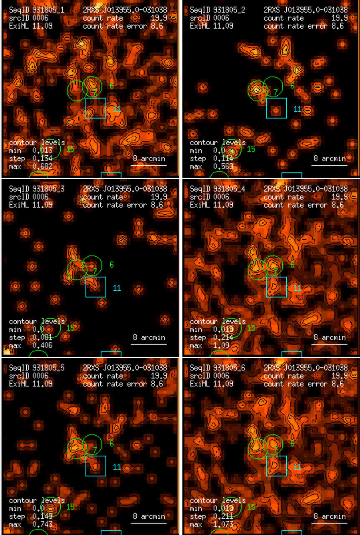
Figure 6: RASS 931805: detection 0006: band rate images, Gaussian filter: (1) PSPC channels 11 – 41, (2) 52 – 90, (3) 91 – 201, (4) 11 – 235, (5) 52 – 201, (6) 11 – 201. Broad band rates in counts/ks. Band rate contour levels in counts/ks/arcmin 2 .
