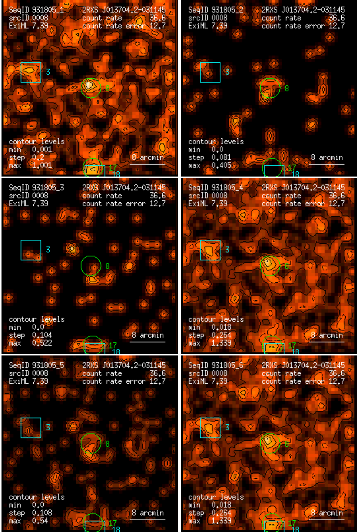
Figure 8: RASS 931805: detection 0008: band rate images, Gaussian filter: (1) PSPC channels 11 – 41, (2) 52 – 90, (3) 91 – 201, (4) 11 – 235, (5) 52 – 201, (6) 11 – 201. Broad band rates in counts/ks. Band rate contour levels in counts/ks/arcmin 2 .
