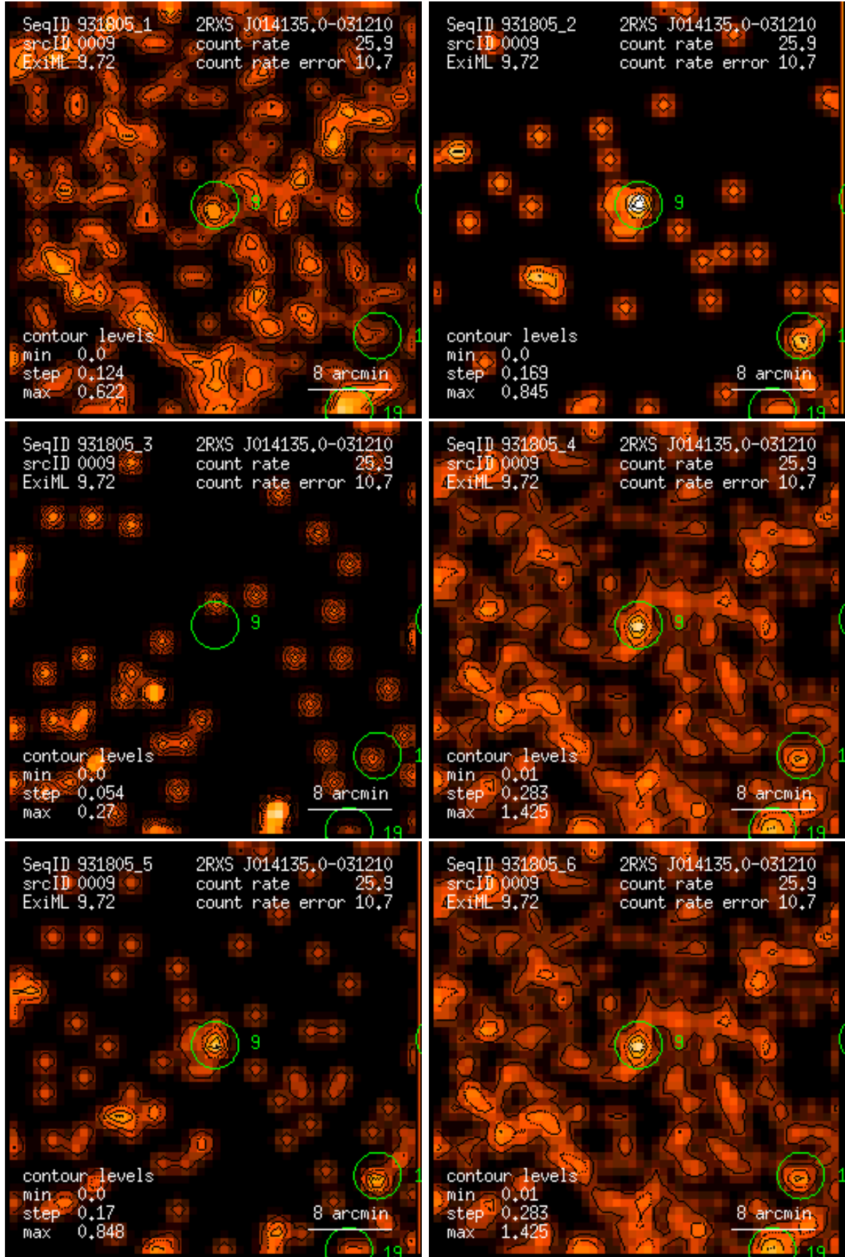
Figure 9: RASS 931805: detection 0009: band rate images, Gaussian filter: (1) PSPC channels 11 – 41, (2) 52 – 90, (3) 91 – 201, (4) 11 – 235, (5) 52 – 201, (6) 11 – 201. Broad band rates in counts/ks. Band rate contour levels in counts/ks/arcmin 2 .
