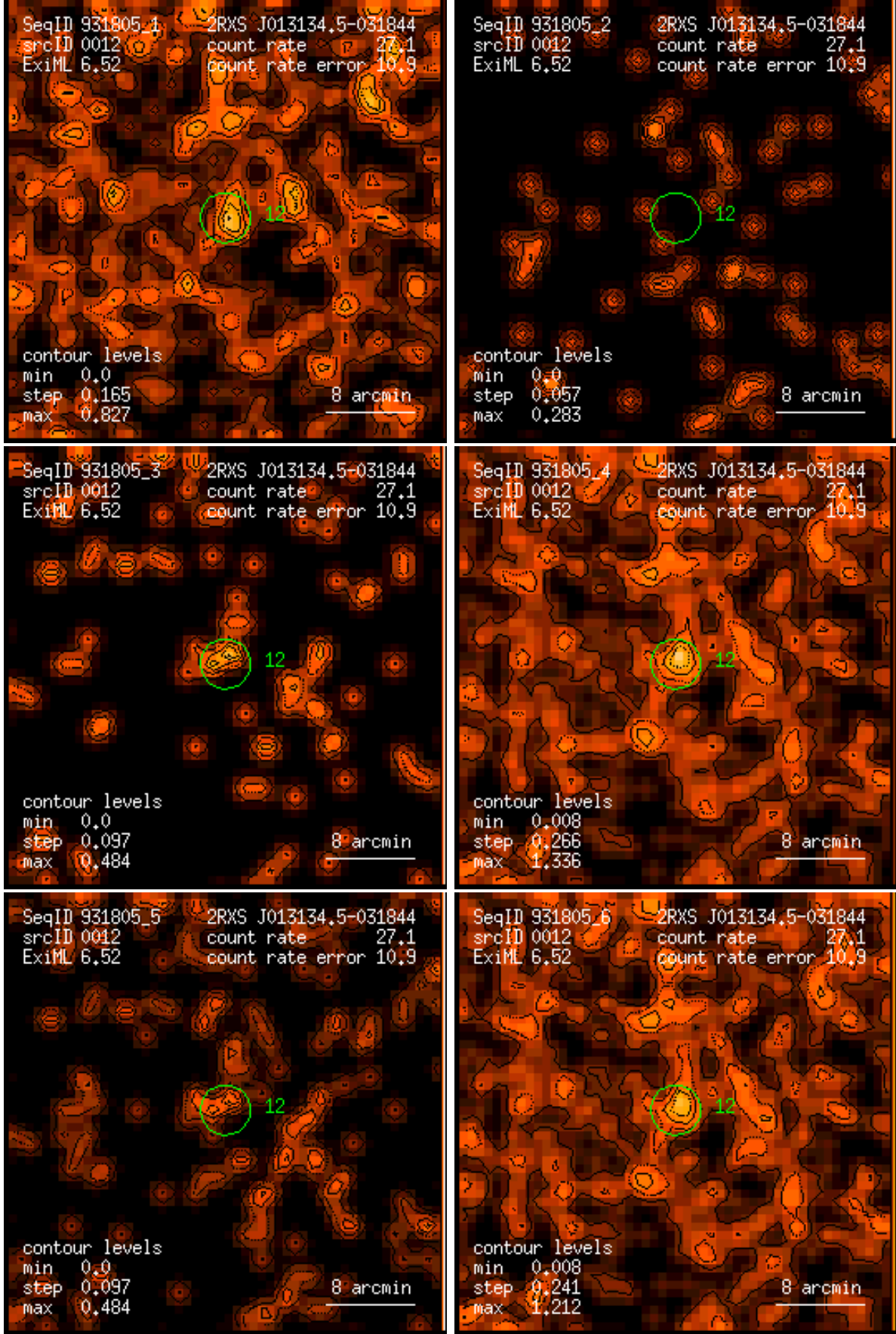
Figure 12: RASS 931805: detection 0012: band rate images, Gaussian filter: (1) PSPC channels 11 – 41, (2) 52 – 90, (3) 91 – 201, (4) 11 – 235, (5) 52 – 201, (6) 11 – 201. Broad band rates in counts/ks. Band rate contour levels in counts/ks/arcmin 2 .
