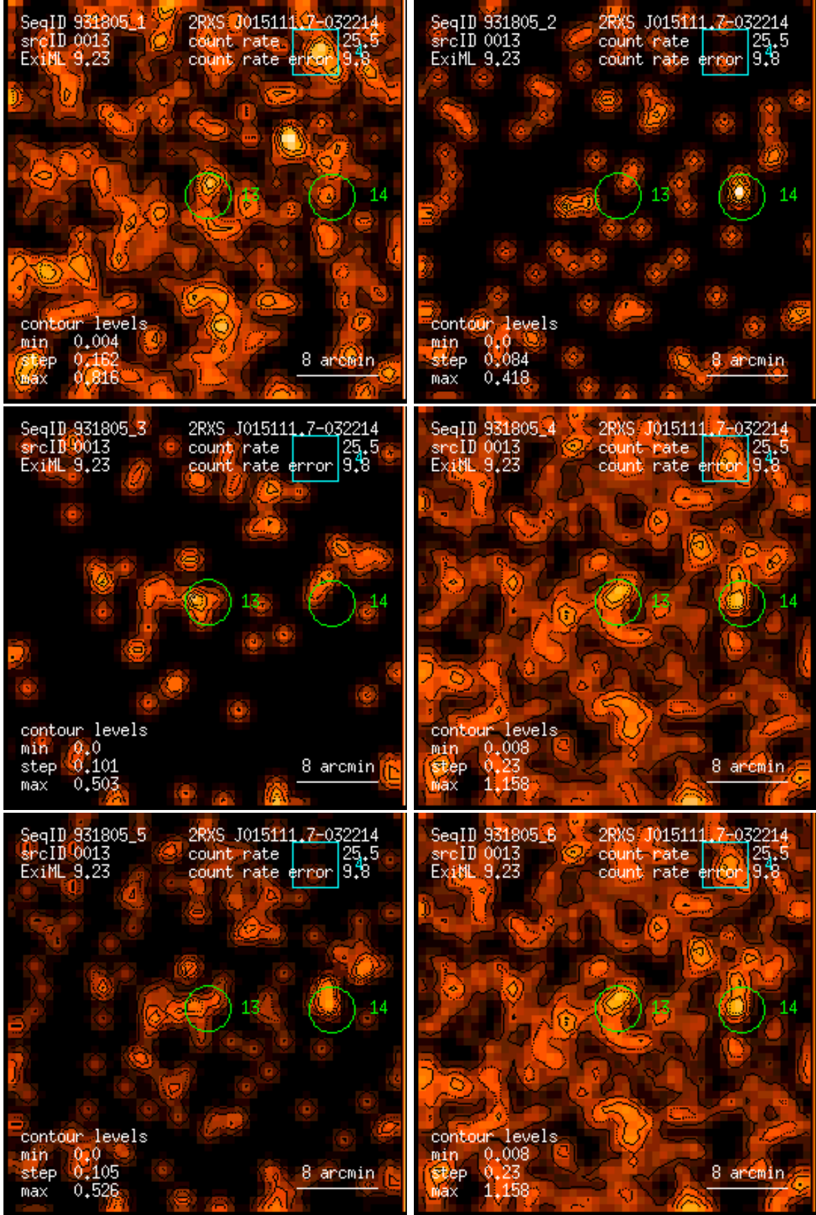
Figure 13: RASS 931805: detection 0013: band rate images, Gaussian filter: (1) PSPC channels 11 – 41, (2) 52 – 90, (3) 91 – 201, (4) 11 – 235, (5) 52 – 201, (6) 11 – 201. Broad band rates in counts/ks. Band rate contour levels in counts/ks/arcmin 2 .
