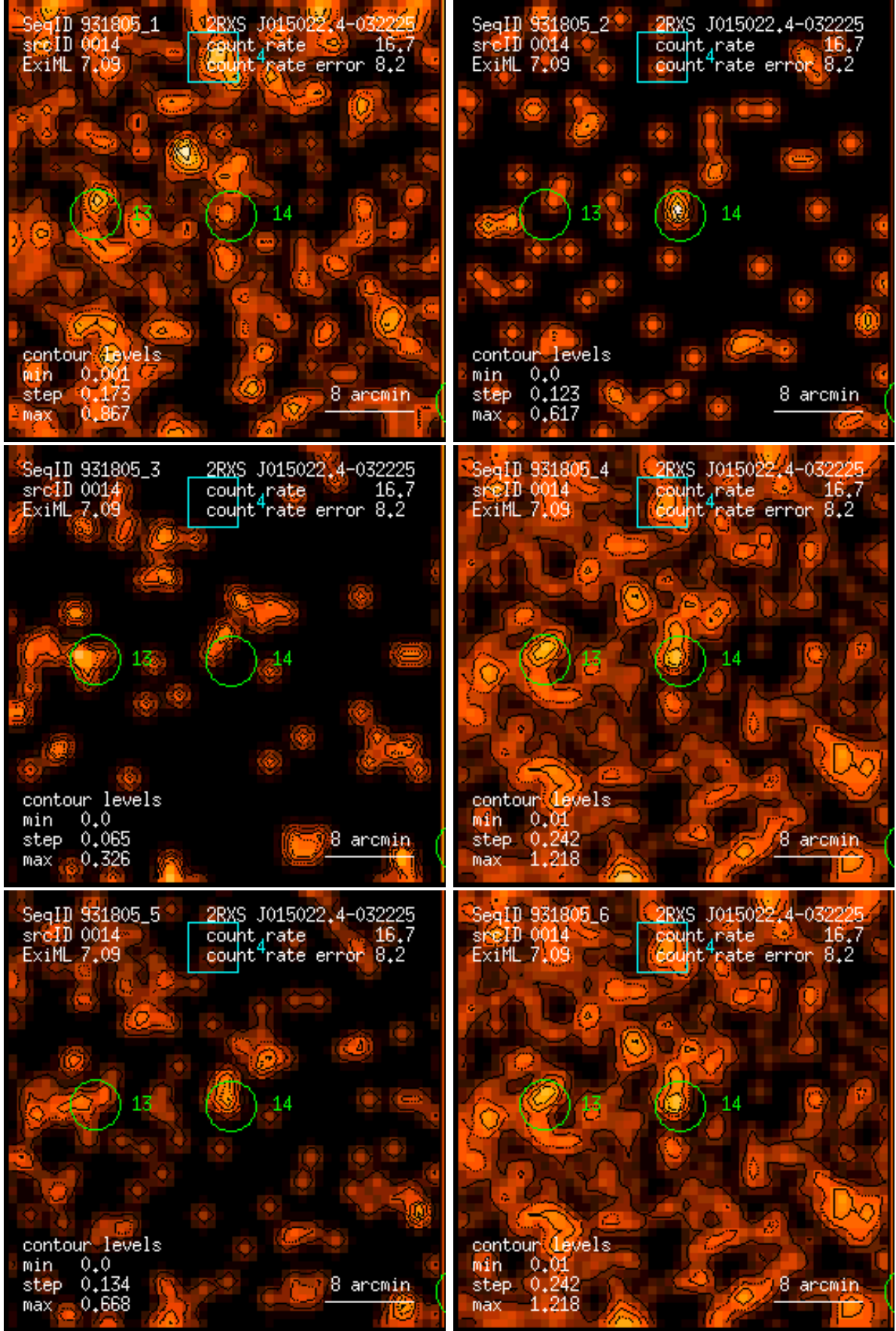
Figure 14: RASS 931805: detection 0014: band rate images, Gaussian filter: (1) PSPC channels 11 – 41, (2) 52 – 90, (3) 91 – 201, (4) 11 – 235, (5) 52 – 201, (6) 11 – 201. Broad band rates in counts/ks. Band rate contour levels in counts/ks/arcmin 2 .
