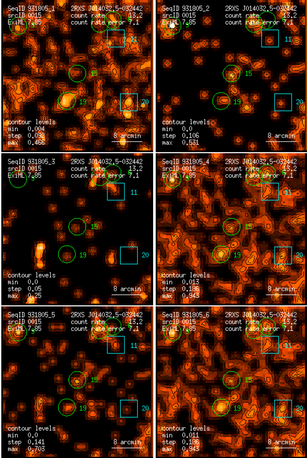
Figure 15: RASS 931805: detection 0015: band rate images, Gaussian filter: (1) PSPC channels 11 – 41, (2) 52 – 90, (3) 91 – 201, (4) 11 – 235, (5) 52 – 201, (6) 11 – 201. Broad band rates in counts/ks. Band rate contour levels in counts/ks/arcmin 2 .
