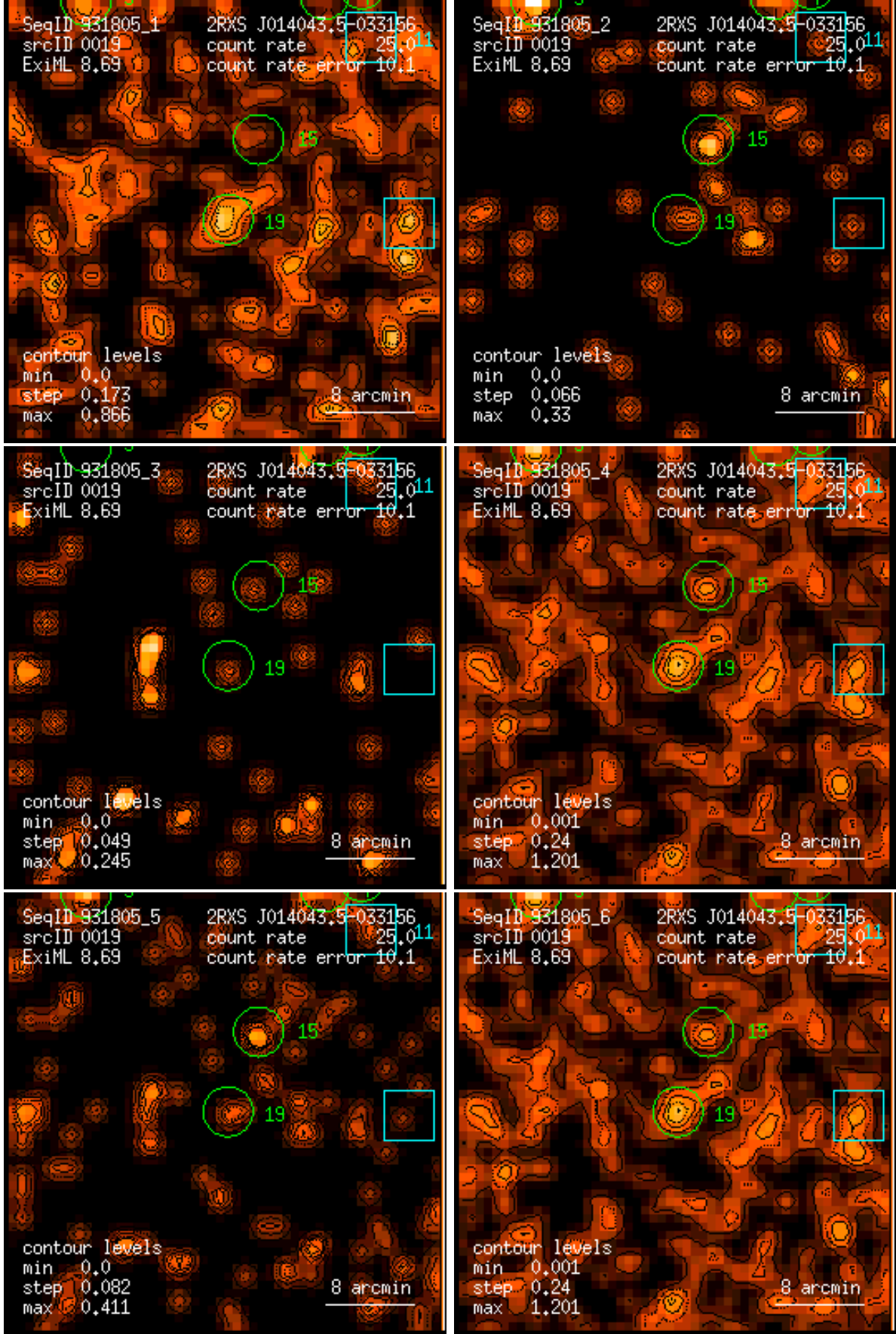
Figure 19: RASS 931805: detection 0019: band rate images, Gaussian filter: (1) PSPC channels 11 – 41, (2) 52 – 90, (3) 91 – 201, (4) 11 – 235, (5) 52 – 201, (6) 11 – 201. Broad band rates in counts/ks. Band rate contour levels in counts/ks/arcmin 2 .
