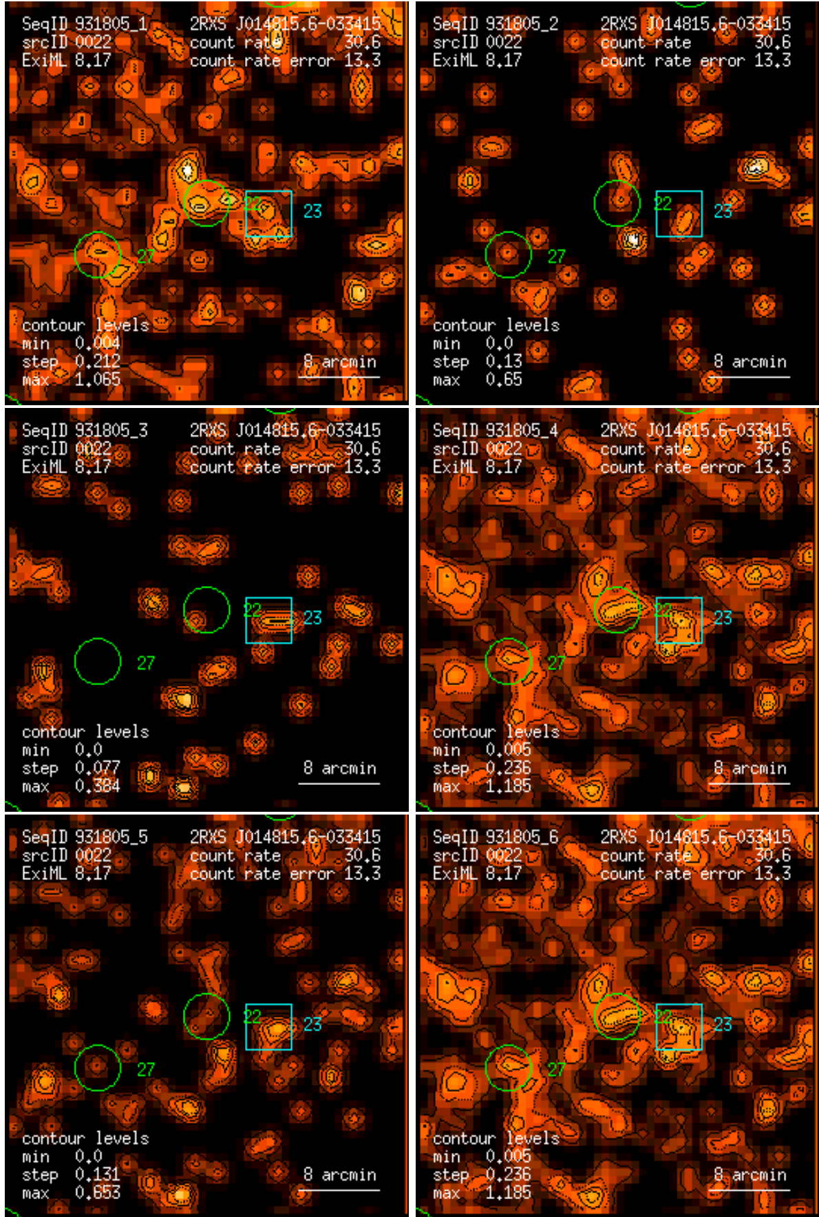
Figure 22: RASS 931805: detection 0022: band rate images, Gaussian filter: (1) PSPC channels 11 – 41, (2) 52 – 90, (3) 91 – 201, (4) 11 – 235, (5) 52 – 201, (6) 11 – 201. Broad band rates in counts/ks. Band rate contour levels in counts/ks/arcmin 2 .
